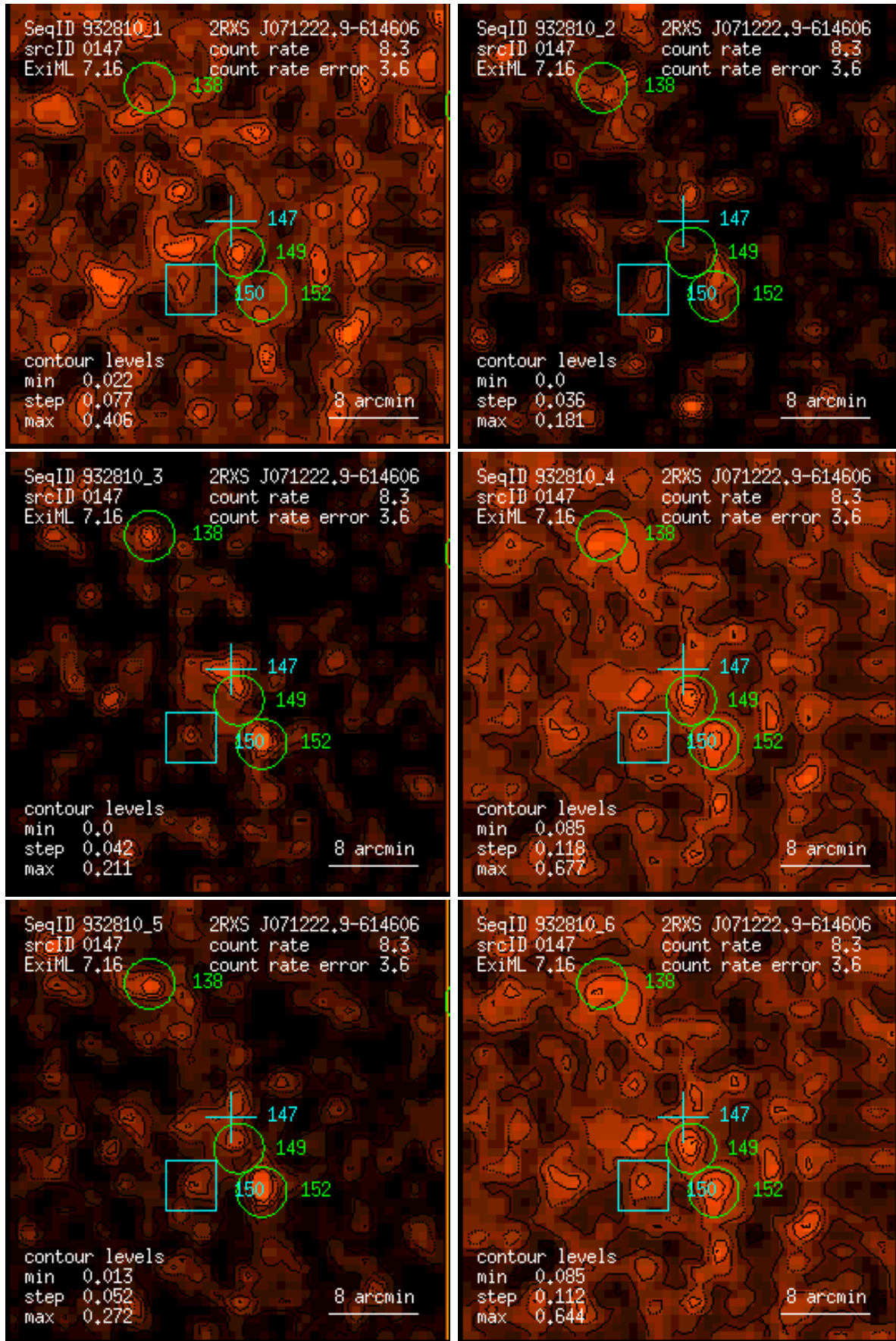
Figure 147: RASS 932810: detection 0147: band rate images, Gaussian filter: (1) PSPC channels 11 – 41, (2) 52 – 90, (3) 91 – 201, (4) 11 – 235, (5) 52 – 201, (6) 11 – 201. Broad band rates in counts/ks. Band rate contour levels in counts/ks/arcmin 2 .
