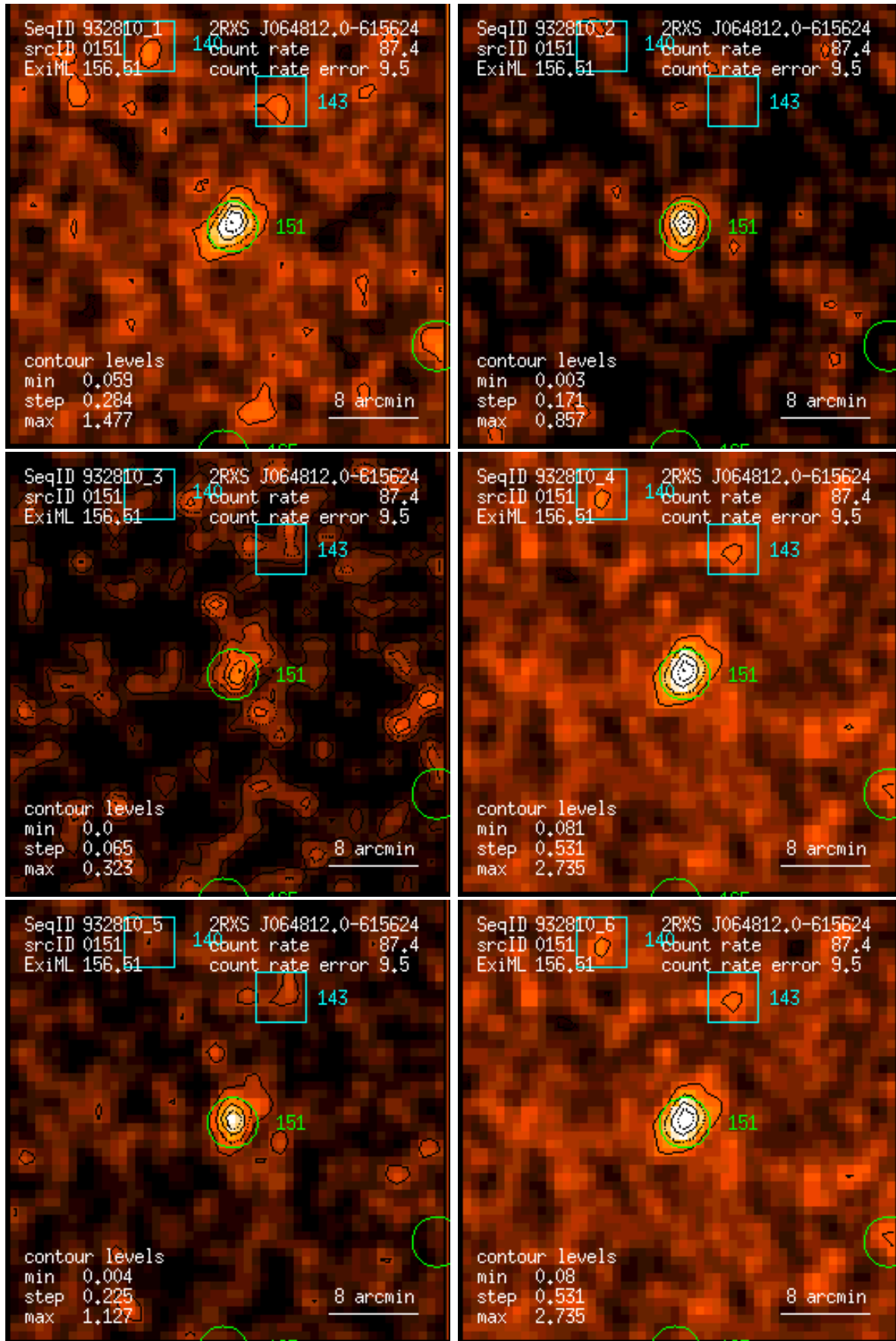
Figure 151: RASS 932810: detection 0151: band rate images, Gaussian filter: (1) PSPC channels 11 – 41, (2) 52 – 90, (3) 91 – 201, (4) 11 – 235, (5) 52 – 201, (6) 11 – 201. Broad band rates in counts/ks. Band rate contour levels in counts/ks/arcmin 2 .
