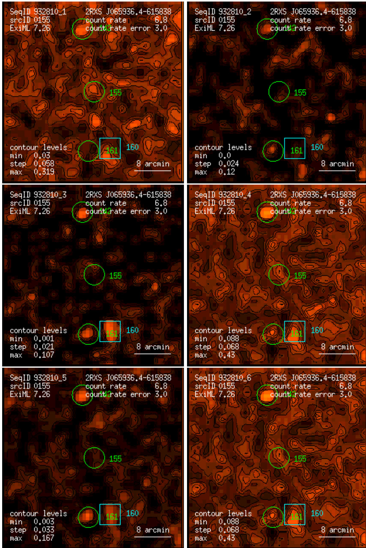
Figure 155: RASS 932810: detection 0155: band rate images, Gaussian filter: (1) PSPC channels 11 – 41, (2) 52 – 90, (3) 91 – 201, (4) 11 – 235, (5) 52 – 201, (6) 11 – 201. Broad band rates in counts/ks. Band rate contour levels in counts/ks/arcmin 2 .
