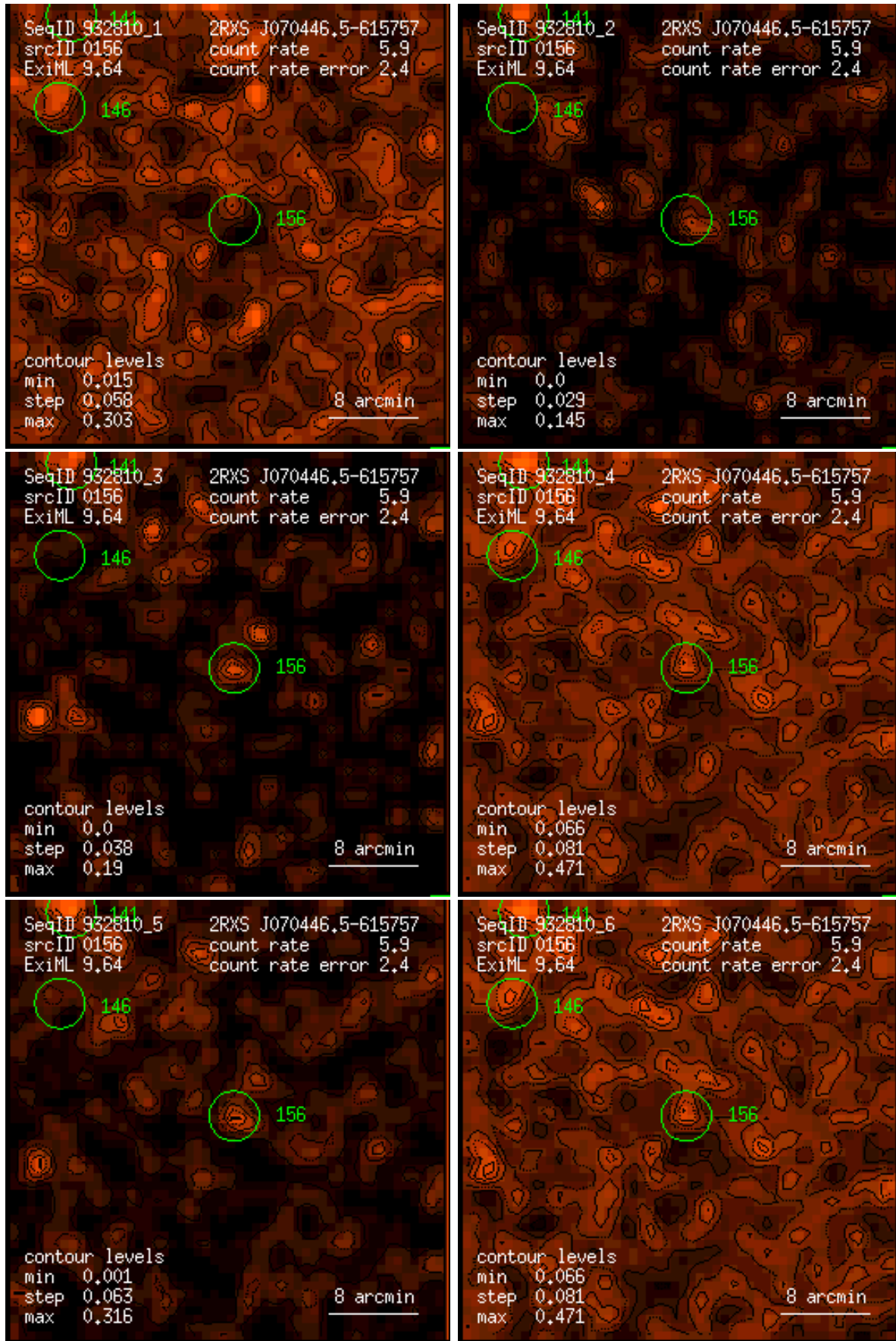
Figure 156: RASS 932810: detection 0156: band rate images, Gaussian filter: (1) PSPC channels 11 – 41, (2) 52 – 90, (3) 91 – 201, (4) 11 – 235, (5) 52 – 201, (6) 11 – 201. Broad band rates in counts/ks. Band rate contour levels in counts/ks/arcmin 2 .
