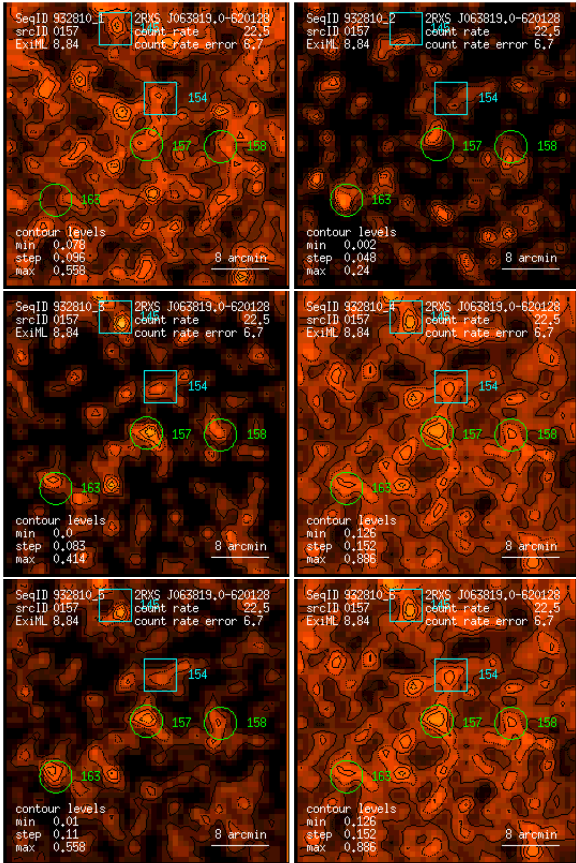
Figure 157: RASS 932810: detection 0157: band rate images, Gaussian filter: (1) PSPC channels 11 – 41, (2) 52 – 90, (3) 91 – 201, (4) 11 – 235, (5) 52 – 201, (6) 11 – 201. Broad band rates in counts/ks. Band rate contour levels in counts/ks/arcmin 2 .
