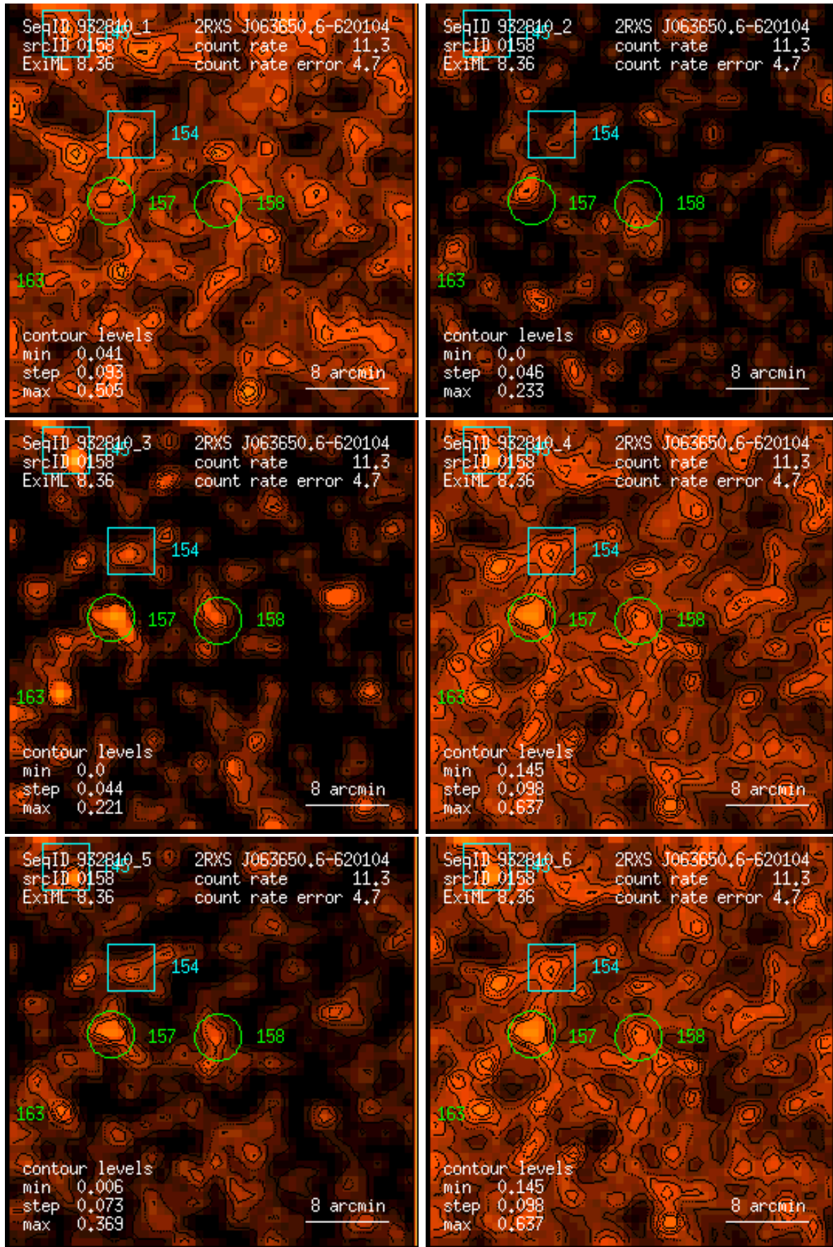
Figure 158: RASS 932810: detection 0158: band rate images, Gaussian filter: (1) PSPC channels 11 – 41, (2) 52 – 90, (3) 91 – 201, (4) 11 – 235, (5) 52 – 201, (6) 11 – 201. Broad band rates in counts/ks. Band rate contour levels in counts/ks/arcmin 2 .
