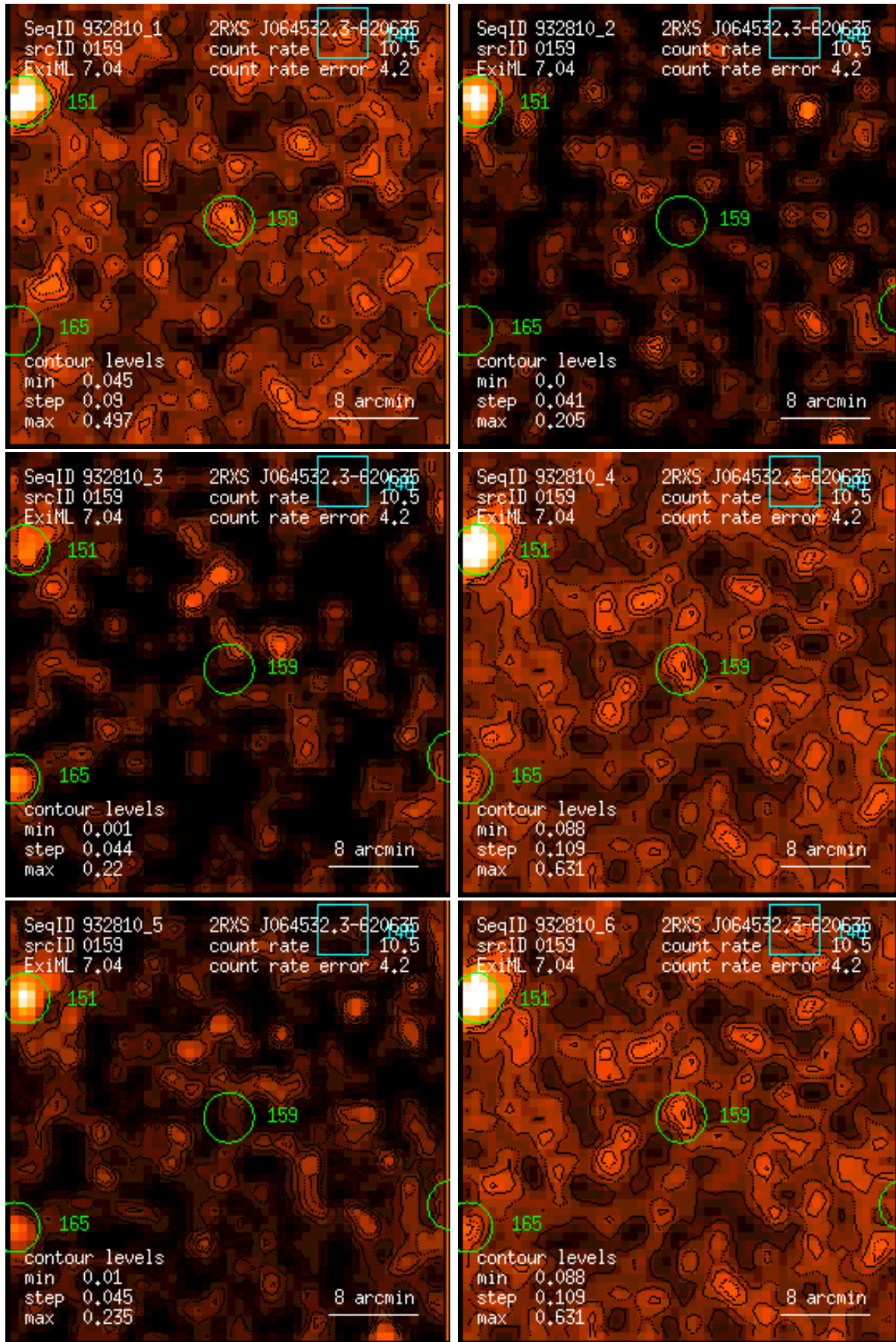
Figure 159: RASS 932810: detection 0159: band rate images, Gaussian filter: (1) PSPC channels 11 – 41, (2) 52 – 90, (3) 91 – 201, (4) 11 – 235, (5) 52 – 201, (6) 11 – 201. Broad band rates in counts/ks. Band rate contour levels in counts/ks/arcmin 2 .
