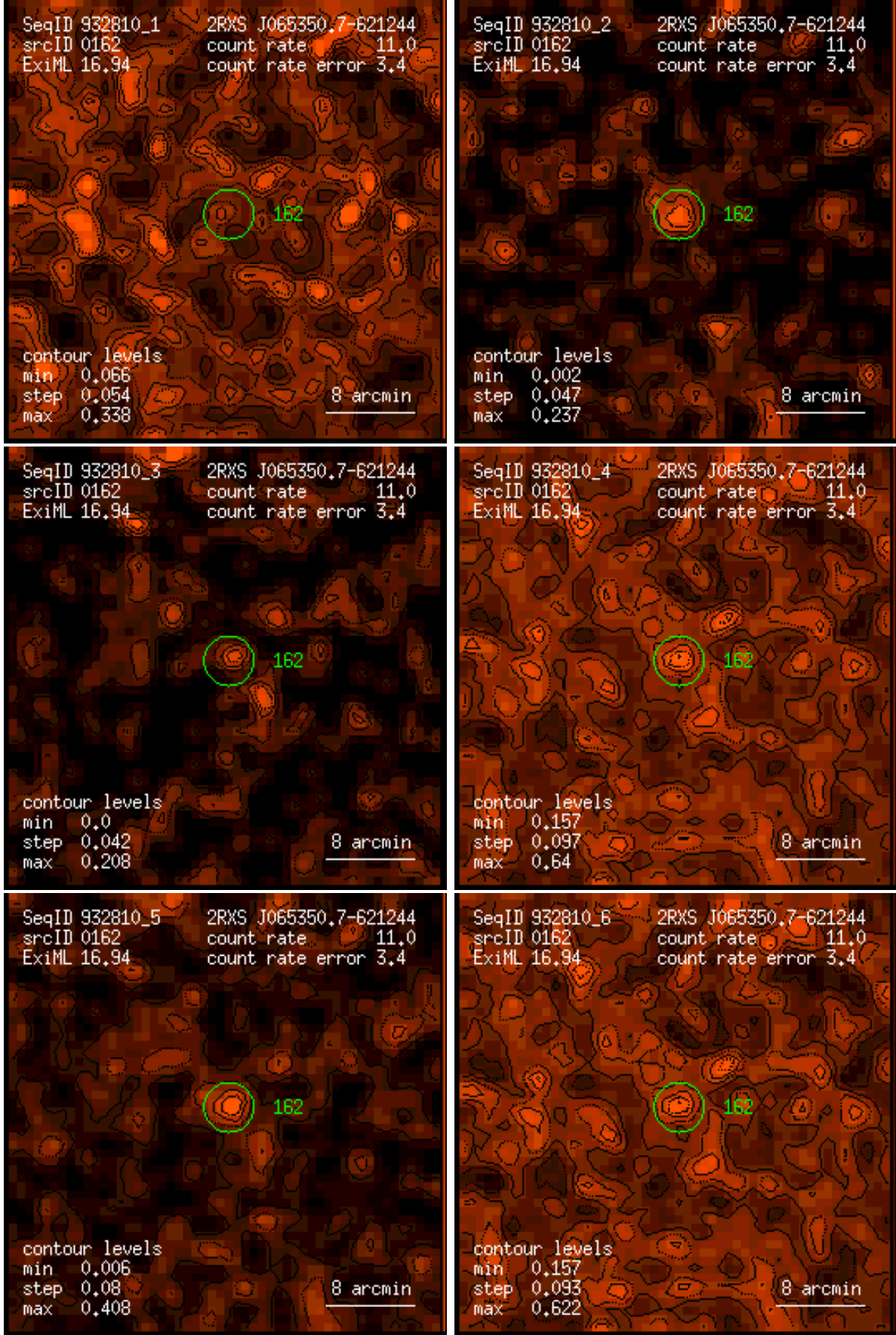
Figure 162: RASS 932810: detection 0162: band rate images, Gaussian filter: (1) PSPC channels 11 – 41, (2) 52 – 90, (3) 91 – 201, (4) 11 – 235, (5) 52 – 201, (6) 11 – 201. Broad band rates in counts/ks. Band rate contour levels in counts/ks/arcmin 2 .
