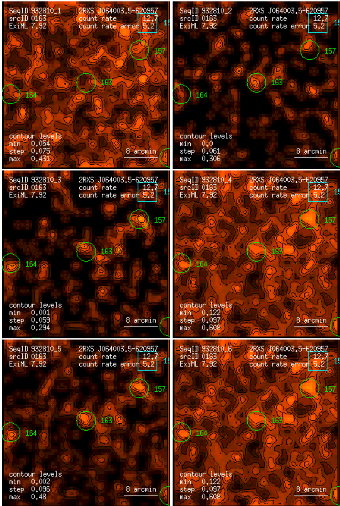
Figure 163: RASS 932810: detection 0163: band rate images, Gaussian filter: (1) PSPC channels 11 – 41, (2) 52 – 90, (3) 91 – 201, (4) 11 – 235, (5) 52 – 201, (6) 11 – 201. Broad band rates in counts/ks. Band rate contour levels in counts/ks/arcmin 2 .
