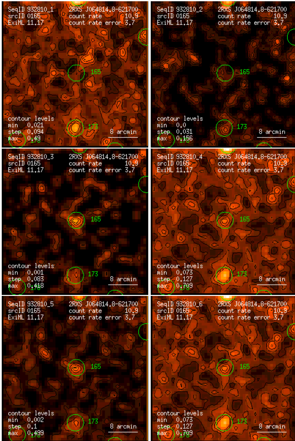
Figure 165: RASS 932810: detection 0165: band rate images, Gaussian filter: (1) PSPC channels 11 – 41, (2) 52 – 90, (3) 91 – 201, (4) 11 – 235, (5) 52 – 201, (6) 11 – 201. Broad band rates in counts/ks. Band rate contour levels in counts/ks/arcmin 2 .
