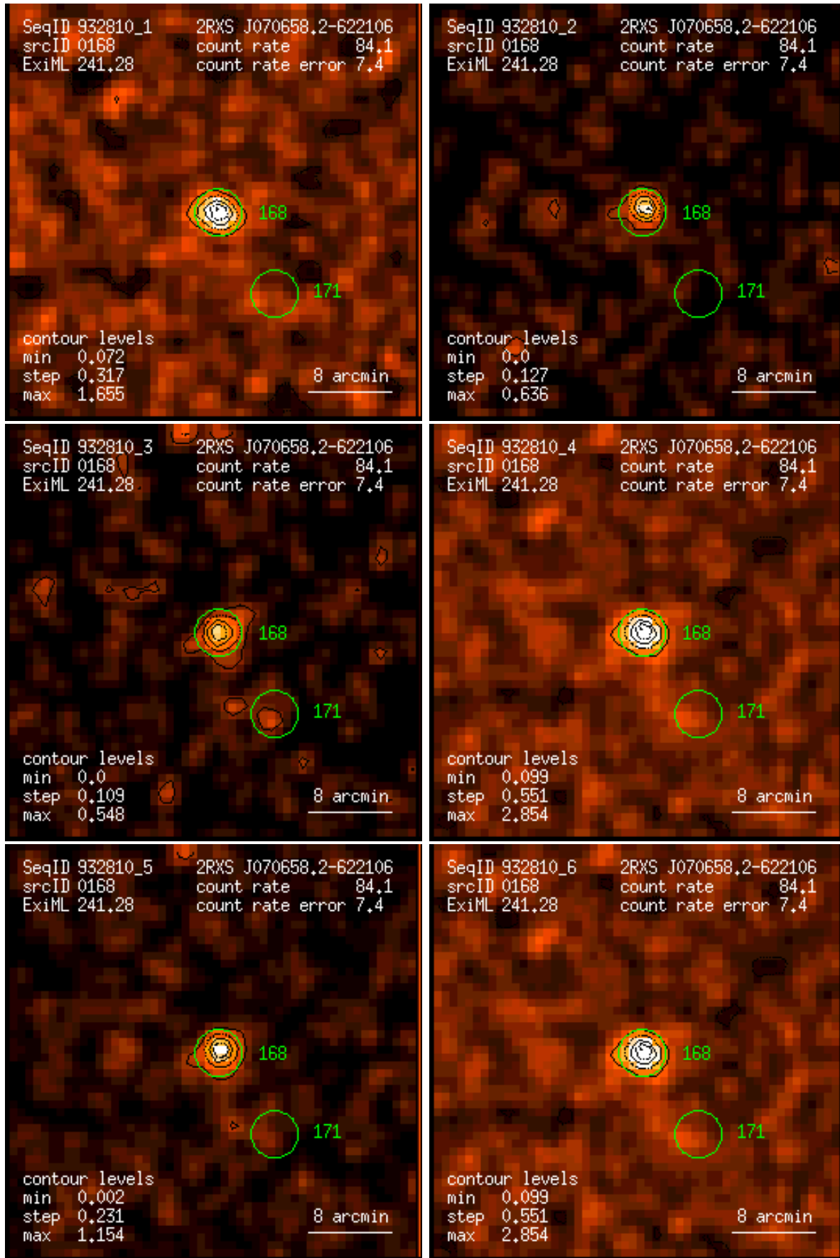
Figure 168: RASS 932810: detection 0168: band rate images, Gaussian filter: (1) PSPC channels 11 – 41, (2) 52 – 90, (3) 91 – 201, (4) 11 – 235, (5) 52 – 201, (6) 11 – 201. Broad band rates in counts/ks. Band rate contour levels in counts/ks/arcmin 2 .
