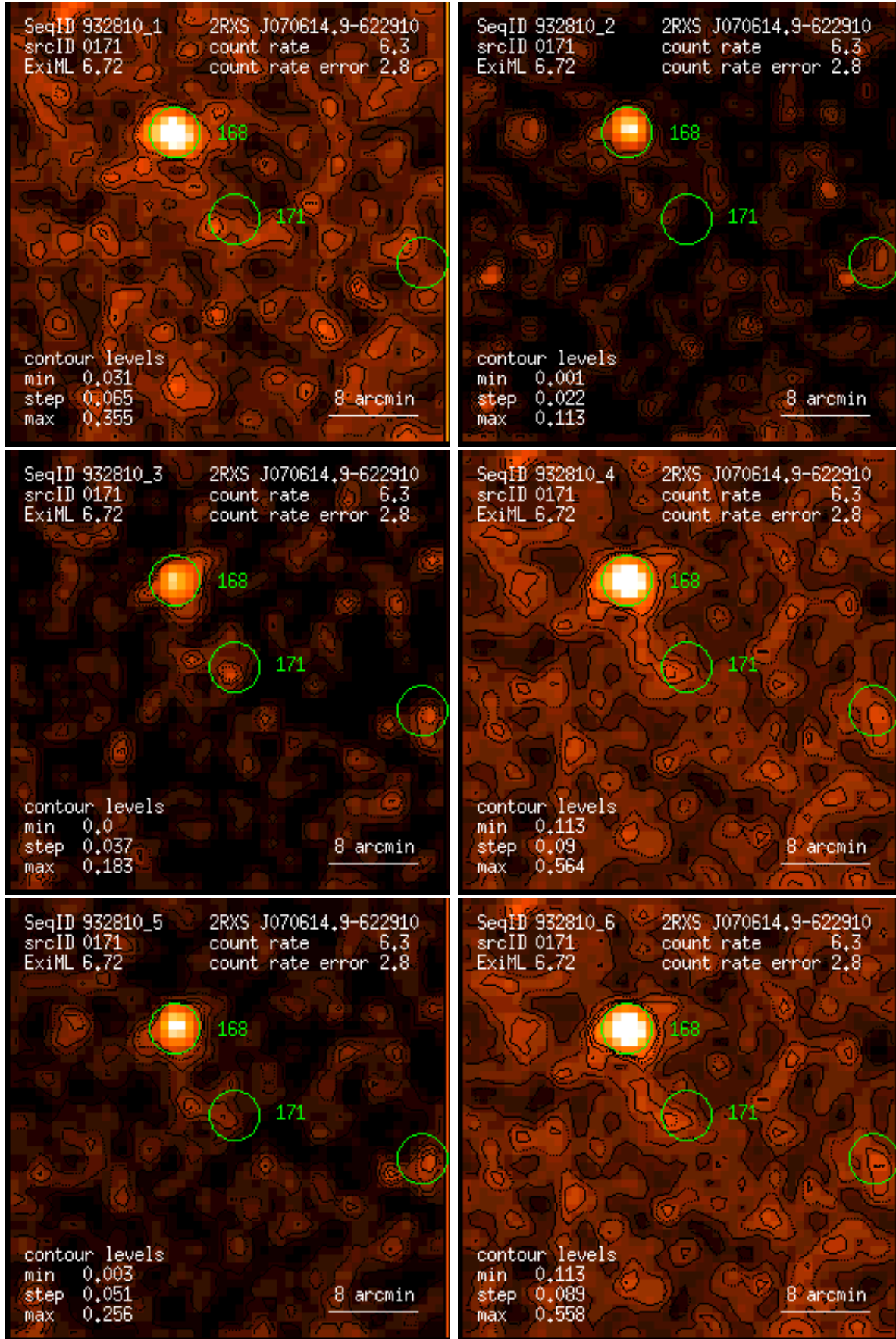
Figure 171: RASS 932810: detection 0171: band rate images, Gaussian filter: (1) PSPC channels 11 – 41, (2) 52 – 90, (3) 91 – 201, (4) 11 – 235, (5) 52 – 201, (6) 11 – 201. Broad band rates in counts/ks. Band rate contour levels in counts/ks/arcmin 2 .
