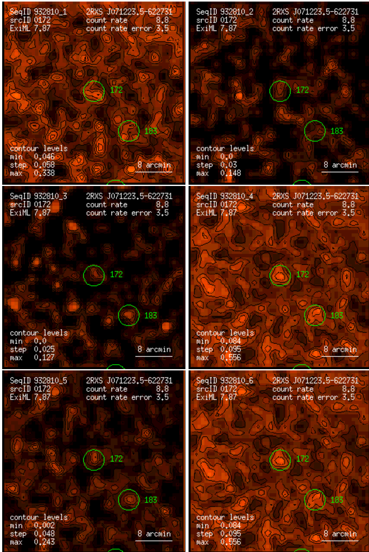
Figure 172: RASS 932810: detection 0172: band rate images, Gaussian filter: (1) PSPC channels 11 – 41, (2) 52 – 90, (3) 91 – 201, (4) 11 – 235, (5) 52 – 201, (6) 11 – 201. Broad band rates in counts/ks. Band rate contour levels in counts/ks/arcmin 2 .
