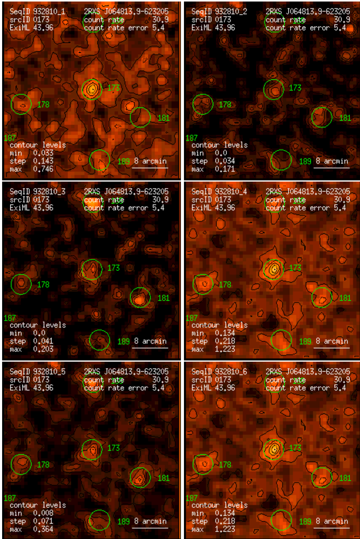
Figure 173: RASS 932810: detection 0173: band rate images, Gaussian filter: (1) PSPC channels 11 – 41, (2) 52 – 90, (3) 91 – 201, (4) 11 – 235, (5) 52 – 201, (6) 11 – 201. Broad band rates in counts/ks. Band rate contour levels in counts/ks/arcmin 2 .
