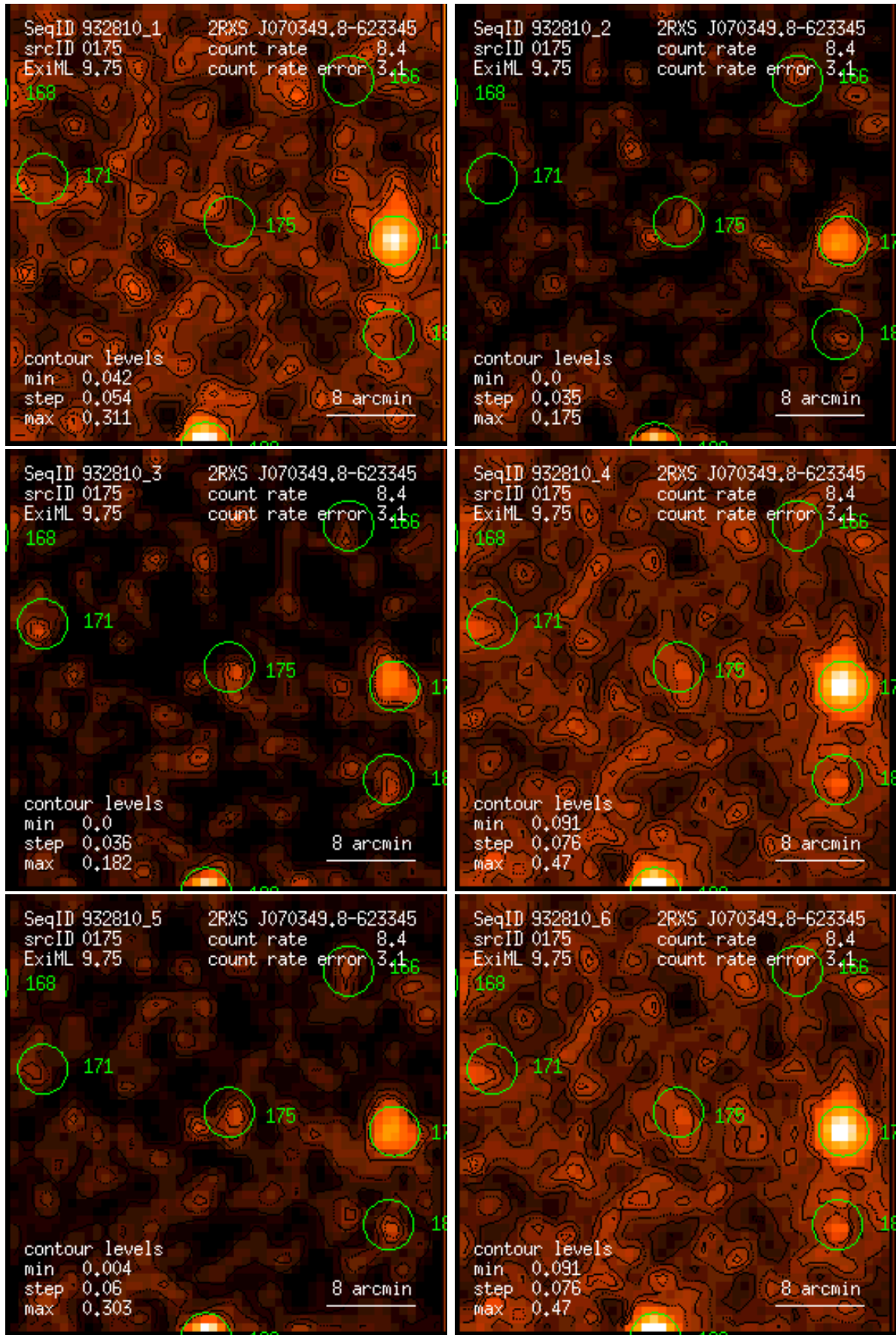
Figure 175: RASS 932810: detection 0175: band rate images, Gaussian filter: (1) PSPC channels 11 – 41, (2) 52 – 90, (3) 91 – 201, (4) 11 – 235, (5) 52 – 201, (6) 11 – 201. Broad band rates in counts/ks. Band rate contour levels in counts/ks/arcmin 2 .
