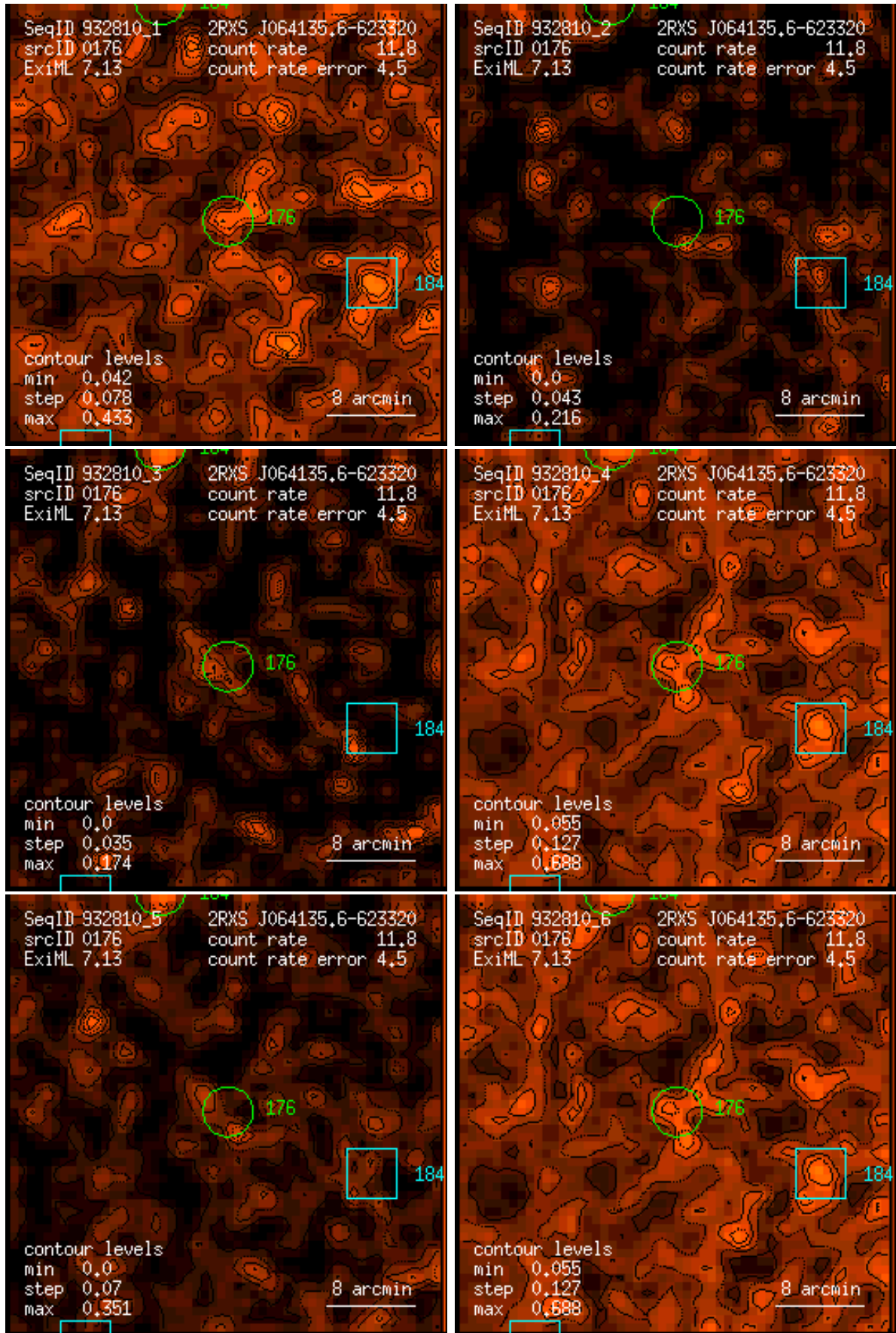
Figure 176: RASS 932810: detection 0176: band rate images, Gaussian filter: (1) PSPC channels 11 – 41, (2) 52 – 90, (3) 91 – 201, (4) 11 – 235, (5) 52 – 201, (6) 11 – 201. Broad band rates in counts/ks. Band rate contour levels in counts/ks/arcmin 2 .
