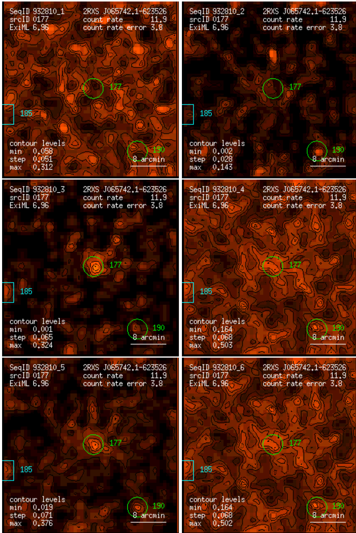
Figure 177: RASS 932810: detection 0177: band rate images, Gaussian filter: (1) PSPC channels 11 – 41, (2) 52 – 90, (3) 91 – 201, (4) 11 – 235, (5) 52 – 201, (6) 11 – 201. Broad band rates in counts/ks. Band rate contour levels in counts/ks/arcmin 2 .
