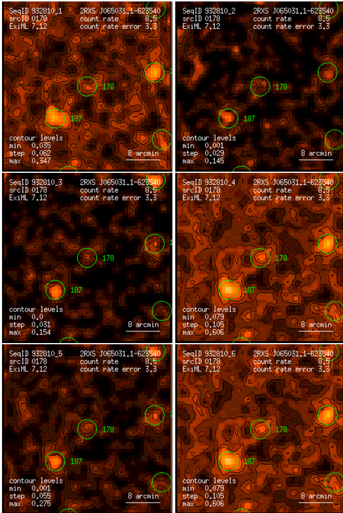
Figure 178: RASS 932810: detection 0178: band rate images, Gaussian filter: (1) PSPC channels 11 – 41, (2) 52 – 90, (3) 91 – 201, (4) 11 – 235, (5) 52 – 201, (6) 11 – 201. Broad band rates in counts/ks. Band rate contour levels in counts/ks/arcmin 2 .
