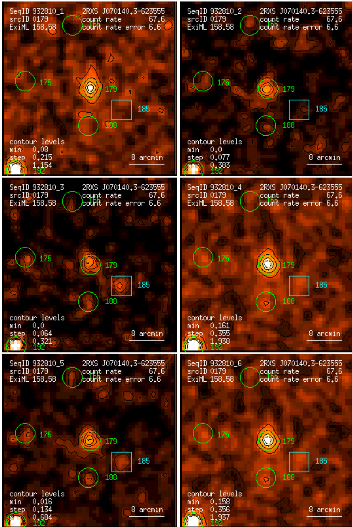
Figure 179: RASS 932810: detection 0179: band rate images, Gaussian filter: (1) PSPC channels 11 – 41, (2) 52 – 90, (3) 91 – 201, (4) 11 – 235, (5) 52 – 201, (6) 11 – 201. Broad band rates in counts/ks. Band rate contour levels in counts/ks/arcmin 2 .
