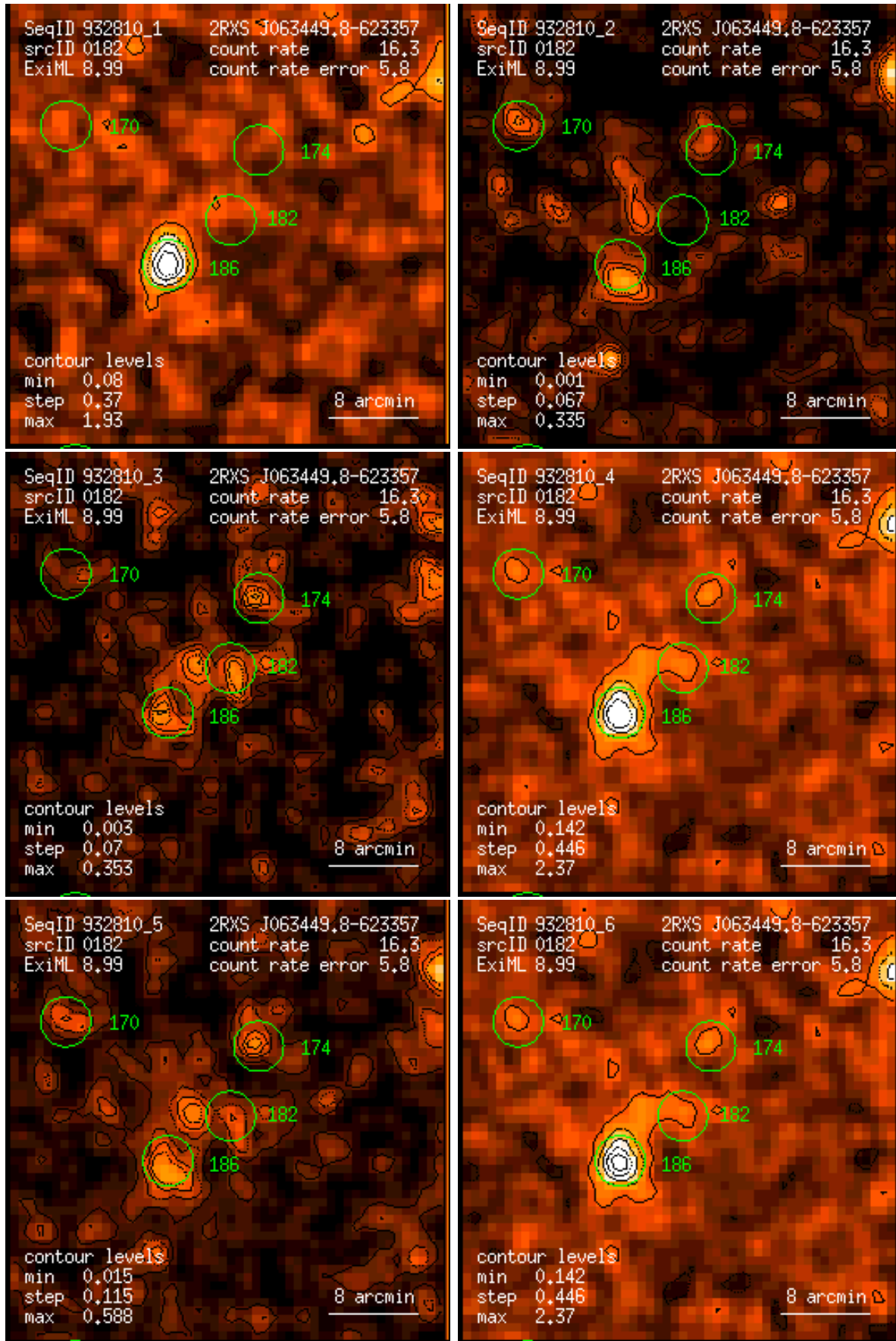
Figure 182: RASS 932810: detection 0182: band rate images, Gaussian filter: (1) PSPC channels 11 – 41, (2) 52 – 90, (3) 91 – 201, (4) 11 – 235, (5) 52 – 201, (6) 11 – 201. Broad band rates in counts/ks. Band rate contour levels in counts/ks/arcmin 2 .
