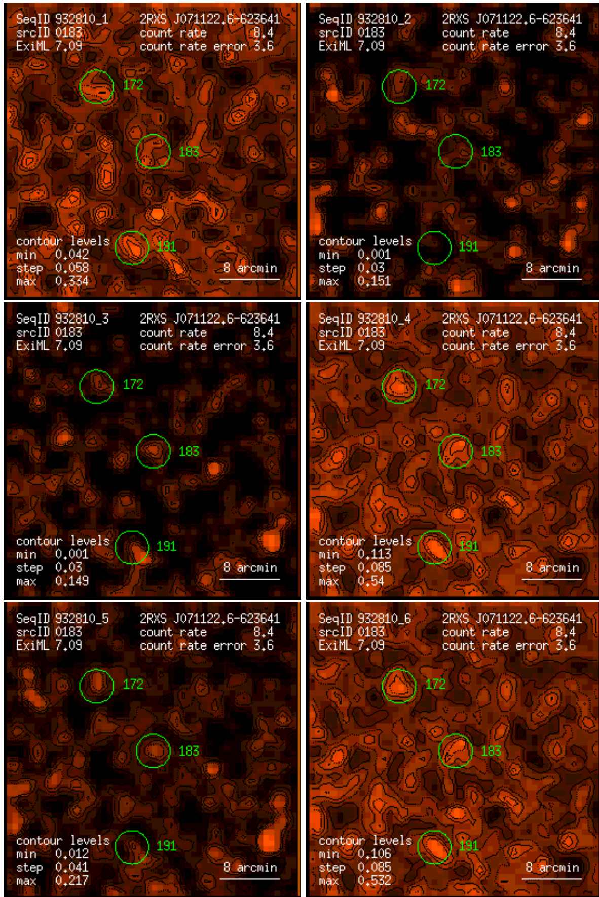
Figure 183: RASS 932810: detection 0183: band rate images, Gaussian filter: (1) PSPC channels 11 – 41, (2) 52 – 90, (3) 91 – 201, (4) 11 – 235, (5) 52 – 201, (6) 11 – 201. Broad band rates in counts/ks. Band rate contour levels in counts/ks/arcmin 2 .
