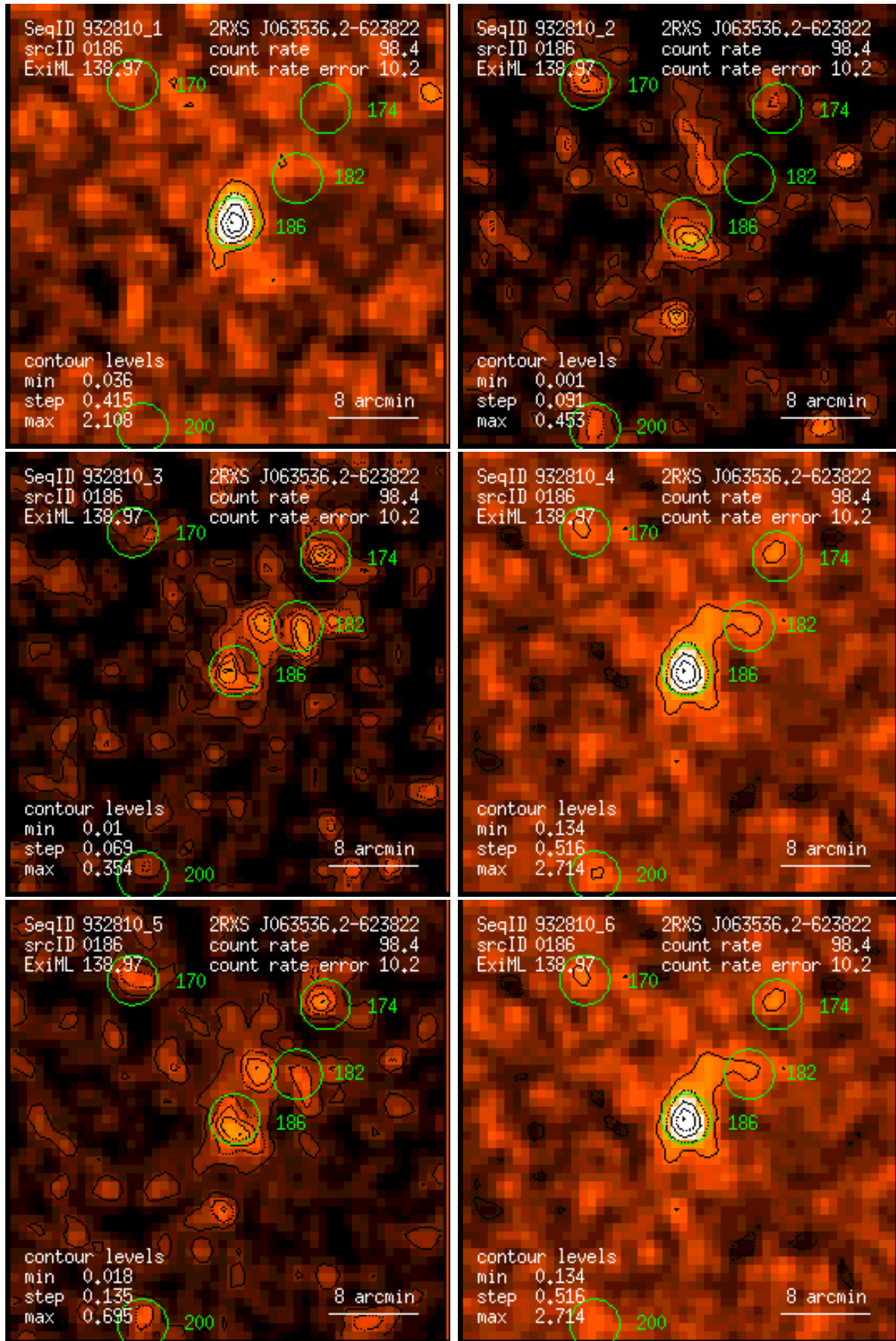
Figure 186: RASS 932810: detection 0186: band rate images, Gaussian filter: (1) PSPC channels 11 – 41, (2) 52 – 90, (3) 91 – 201, (4) 11 – 235, (5) 52 – 201, (6) 11 – 201. Broad band rates in counts/ks. Band rate contour levels in counts/ks/arcmin 2 .
