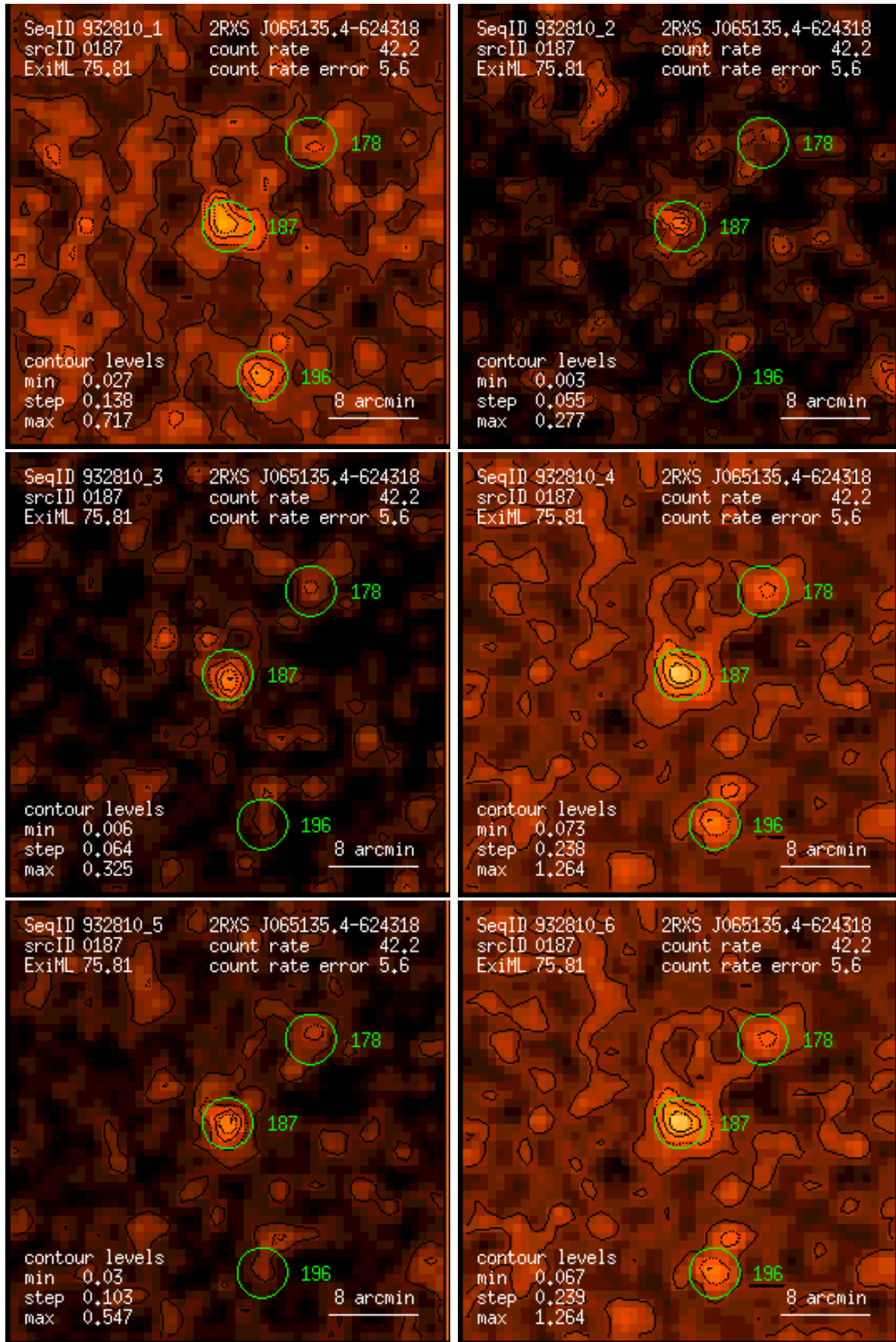
Figure 187: RASS 932810: detection 0187: band rate images, Gaussian filter: (1) PSPC channels 11 – 41, (2) 52 – 90, (3) 91 – 201, (4) 11 – 235, (5) 52 – 201, (6) 11 – 201. Broad band rates in counts/ks. Band rate contour levels in counts/ks/arcmin 2 .
