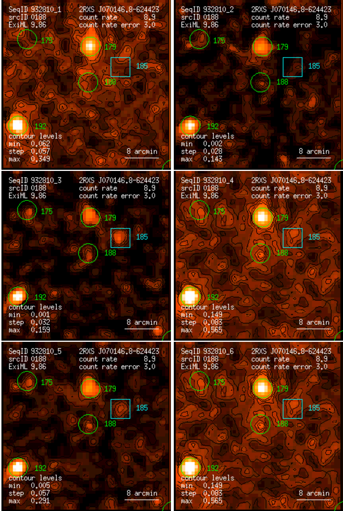
Figure 188: RASS 932810: detection 0188: band rate images, Gaussian filter: (1) PSPC channels 11 – 41, (2) 52 – 90, (3) 91 – 201, (4) 11 – 235, (5) 52 – 201, (6) 11 – 201. Broad band rates in counts/ks. Band rate contour levels in counts/ks/arcmin 2 .
