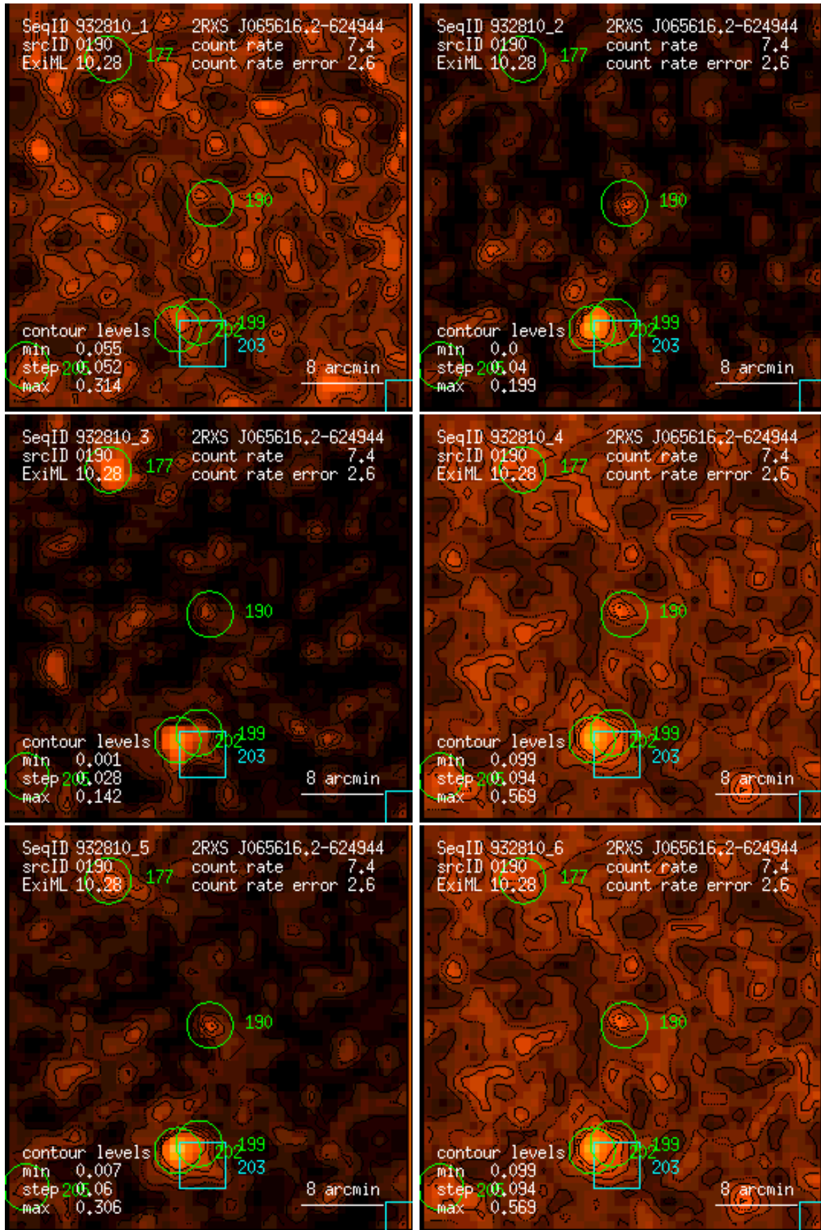
Figure 190: RASS 932810: detection 0190: band rate images, Gaussian filter: (1) PSPC channels 11 – 41, (2) 52 – 90, (3) 91 – 201, (4) 11 – 235, (5) 52 – 201, (6) 11 – 201. Broad band rates in counts/ks. Band rate contour levels in counts/ks/arcmin 2 .
