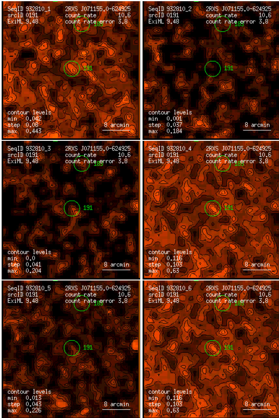
Figure 191: RASS 932810: detection 0191: band rate images, Gaussian filter: (1) PSPC channels 11 – 41, (2) 52 – 90, (3) 91 – 201, (4) 11 – 235, (5) 52 – 201, (6) 11 – 201. Broad band rates in counts/ks. Band rate contour levels in counts/ks/arcmin 2 .
