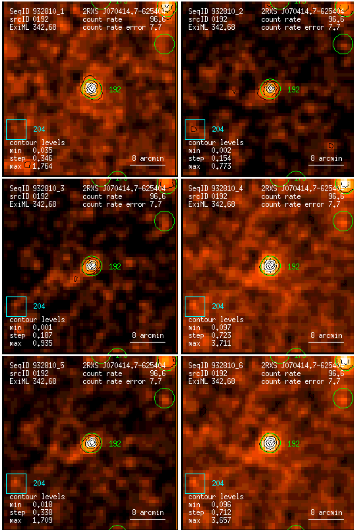
Figure 192: RASS 932810: detection 0192: band rate images, Gaussian filter: (1) PSPC channels 11 – 41, (2) 52 – 90, (3) 91 – 201, (4) 11 – 235, (5) 52 – 201, (6) 11 – 201. Broad band rates in counts/ks. Band rate contour levels in counts/ks/arcmin 2 .
