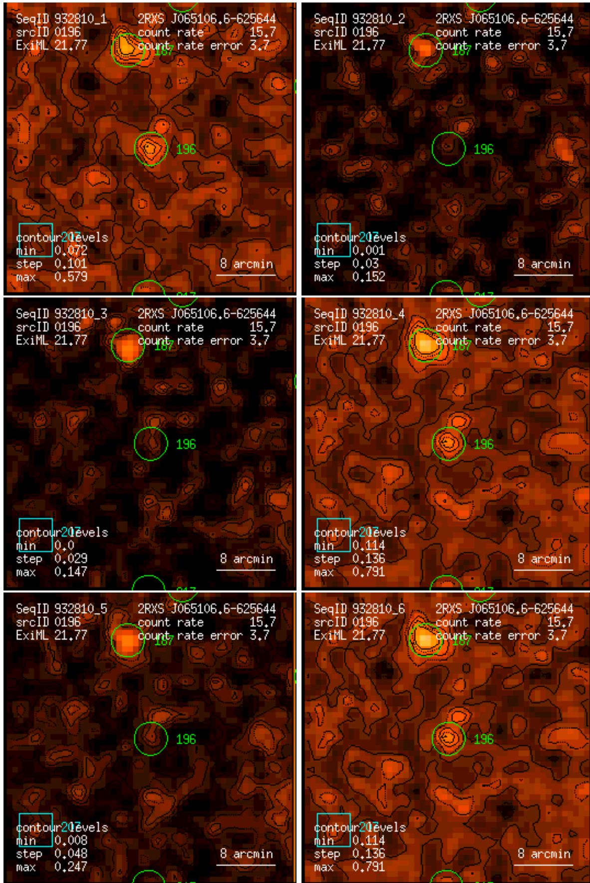
Figure 196: RASS 932810: detection 0196: band rate images, Gaussian filter: (1) PSPC channels 11 – 41, (2) 52 – 90, (3) 91 – 201, (4) 11 – 235, (5) 52 – 201, (6) 11 – 201. Broad band rates in counts/ks. Band rate contour levels in counts/ks/arcmin 2 .
