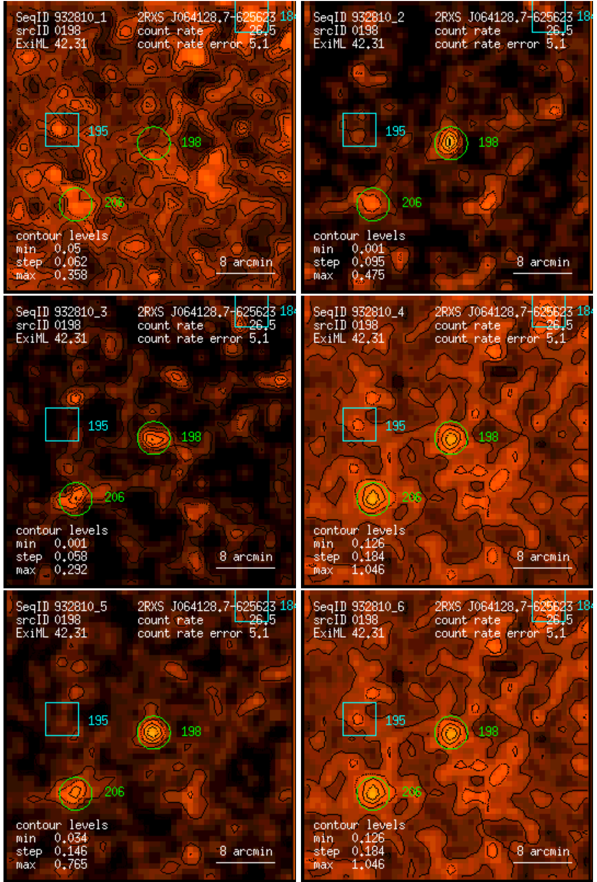
Figure 198: RASS 932810: detection 0198: band rate images, Gaussian filter: (1) PSPC channels 11 – 41, (2) 52 – 90, (3) 91 – 201, (4) 11 – 235, (5) 52 – 201, (6) 11 – 201. Broad band rates in counts/ks. Band rate contour levels in counts/ks/arcmin 2 .
