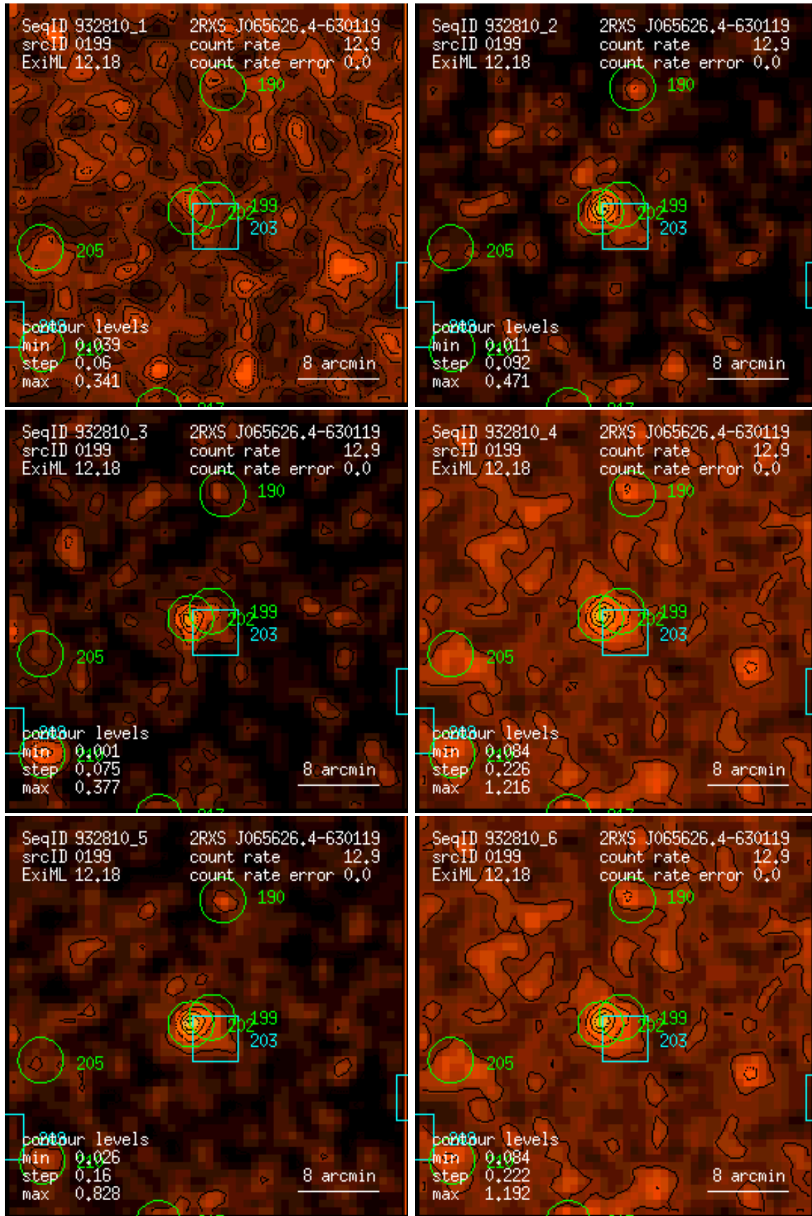
Figure 199: RASS 932810: detection 0199: band rate images, Gaussian filter: (1) PSPC channels 11 – 41, (2) 52 – 90, (3) 91 – 201, (4) 11 – 235, (5) 52 – 201, (6) 11 – 201. Broad band rates in counts/ks. Band rate contour levels in counts/ks/arcmin 2 .
