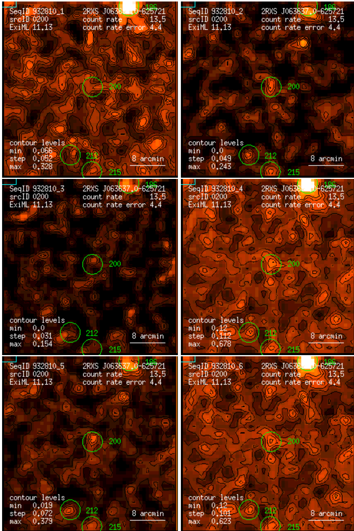
Figure 200: RASS 932810: detection 0200: band rate images, Gaussian filter: (1) PSPC channels 11 – 41, (2) 52 – 90, (3) 91 – 201, (4) 11 – 235, (5) 52 – 201, (6) 11 – 201. Broad band rates in counts/ks. Band rate contour levels in counts/ks/arcmin 2 .
