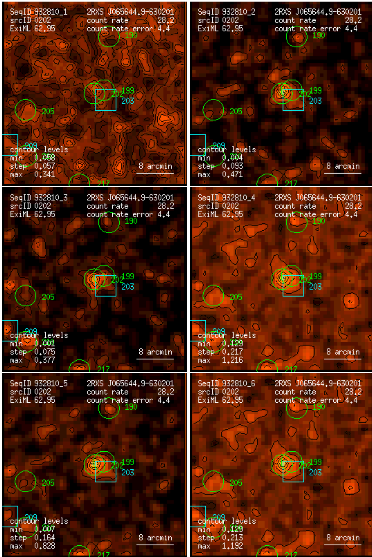
Figure 202: RASS 932810: detection 0202: band rate images, Gaussian filter: (1) PSPC channels 11 – 41, (2) 52 – 90, (3) 91 – 201, (4) 11 – 235, (5) 52 – 201, (6) 11 – 201. Broad band rates in counts/ks. Band rate contour levels in counts/ks/arcmin 2 .
