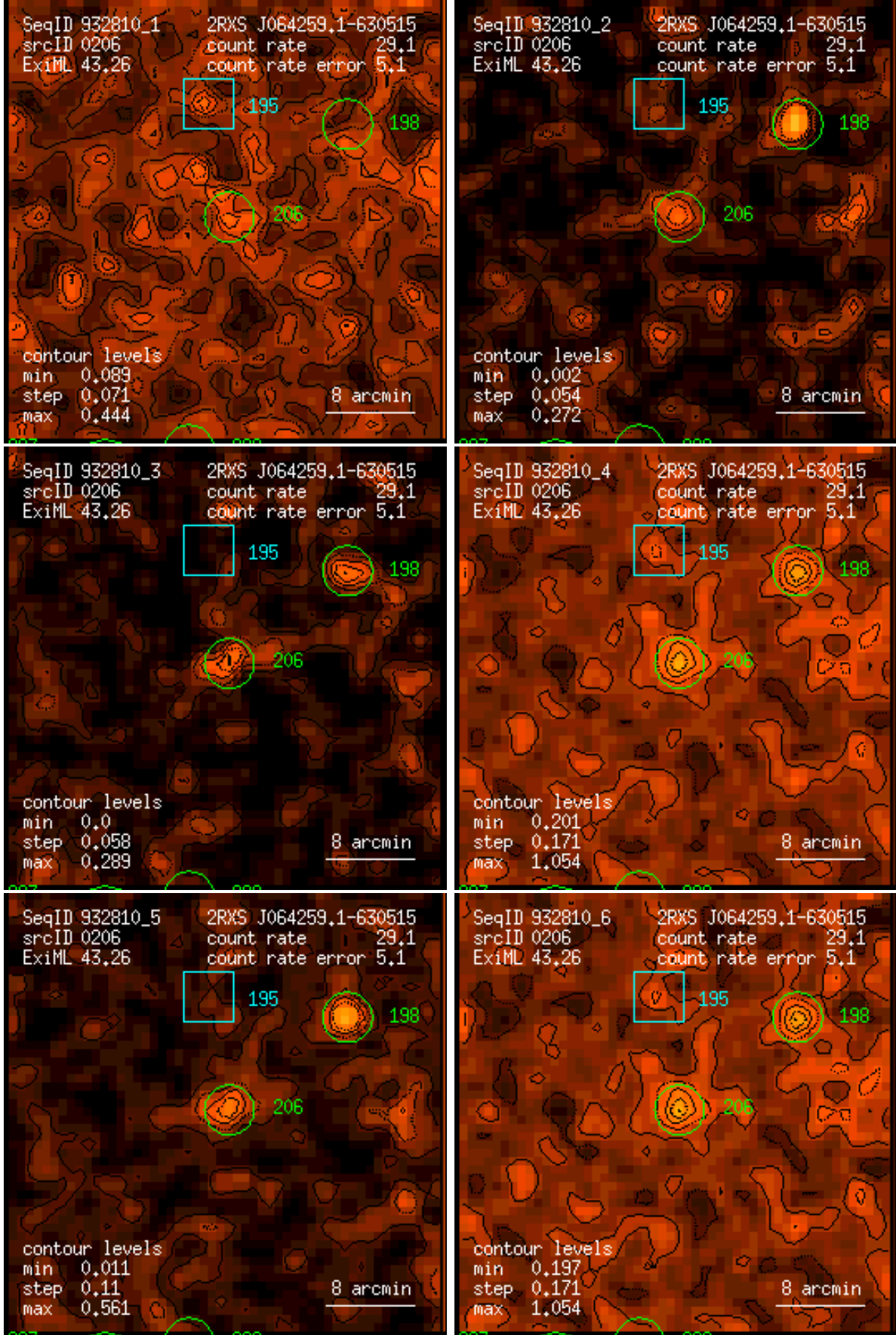
Figure 206: RASS 932810: detection 0206: band rate images, Gaussian filter: (1) PSPC channels 11 – 41, (2) 52 – 90, (3) 91 – 201, (4) 11 – 235, (5) 52 – 201, (6) 11 – 201. Broad band rates in counts/ks. Band rate contour levels in counts/ks/arcmin 2 .
