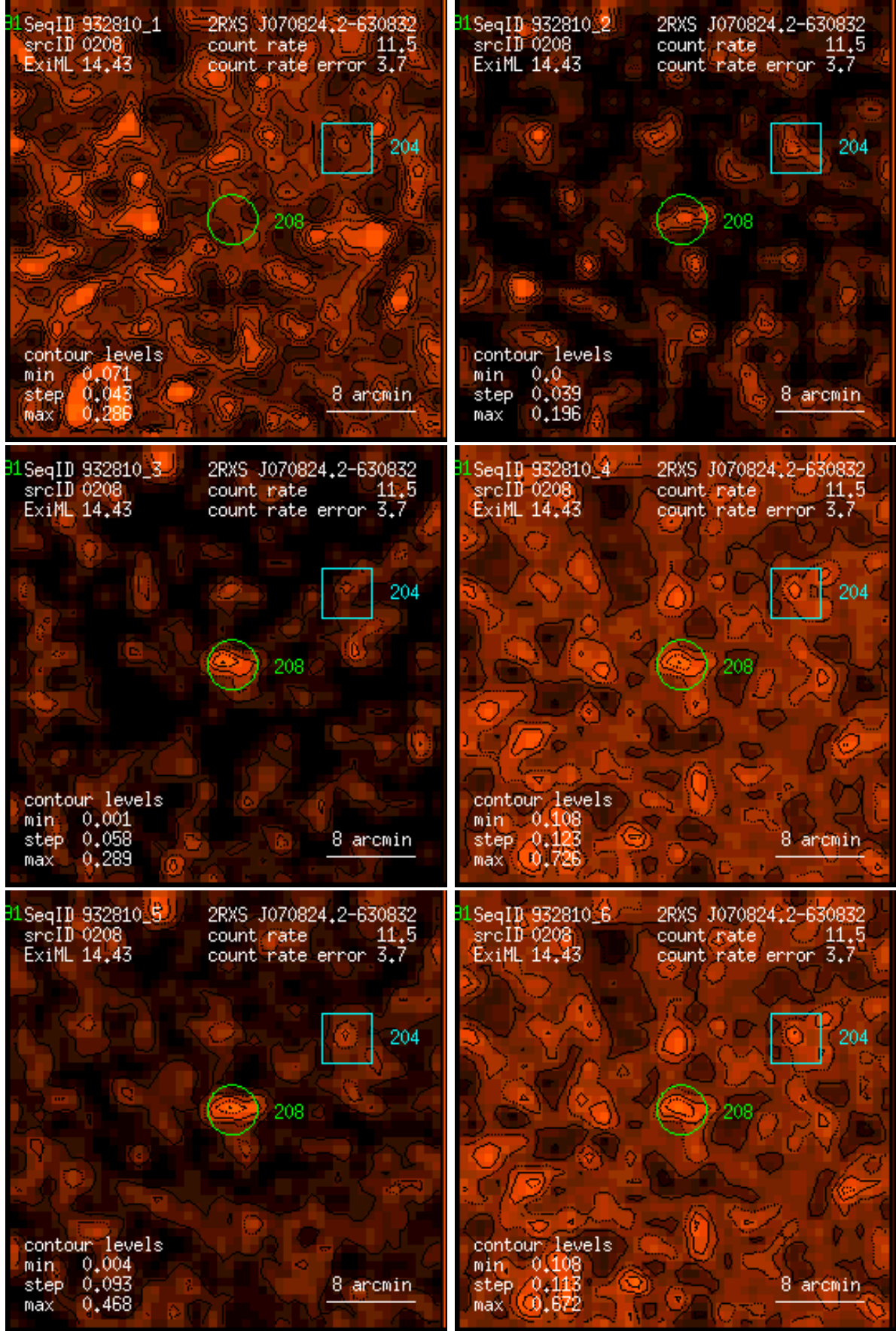
Figure 208: RASS 932810: detection 0208: band rate images, Gaussian filter: (1) PSPC channels 11 – 41, (2) 52 – 90, (3) 91 – 201, (4) 11 – 235, (5) 52 – 201, (6) 11 – 201. Broad band rates in counts/ks. Band rate contour levels in counts/ks/arcmin 2 .
