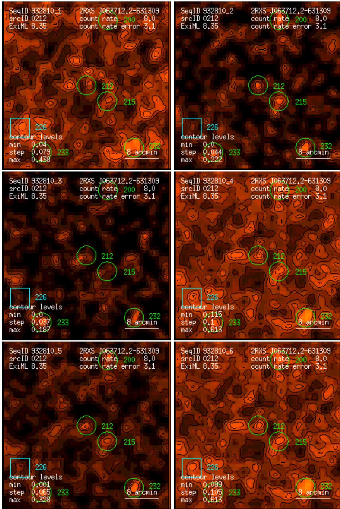
Figure 212: RASS 932810: detection 0212: band rate images, Gaussian filter: (1) PSPC channels 11 – 41, (2) 52 – 90, (3) 91 – 201, (4) 11 – 235, (5) 52 – 201, (6) 11 – 201. Broad band rates in counts/ks. Band rate contour levels in counts/ks/arcmin 2 .
