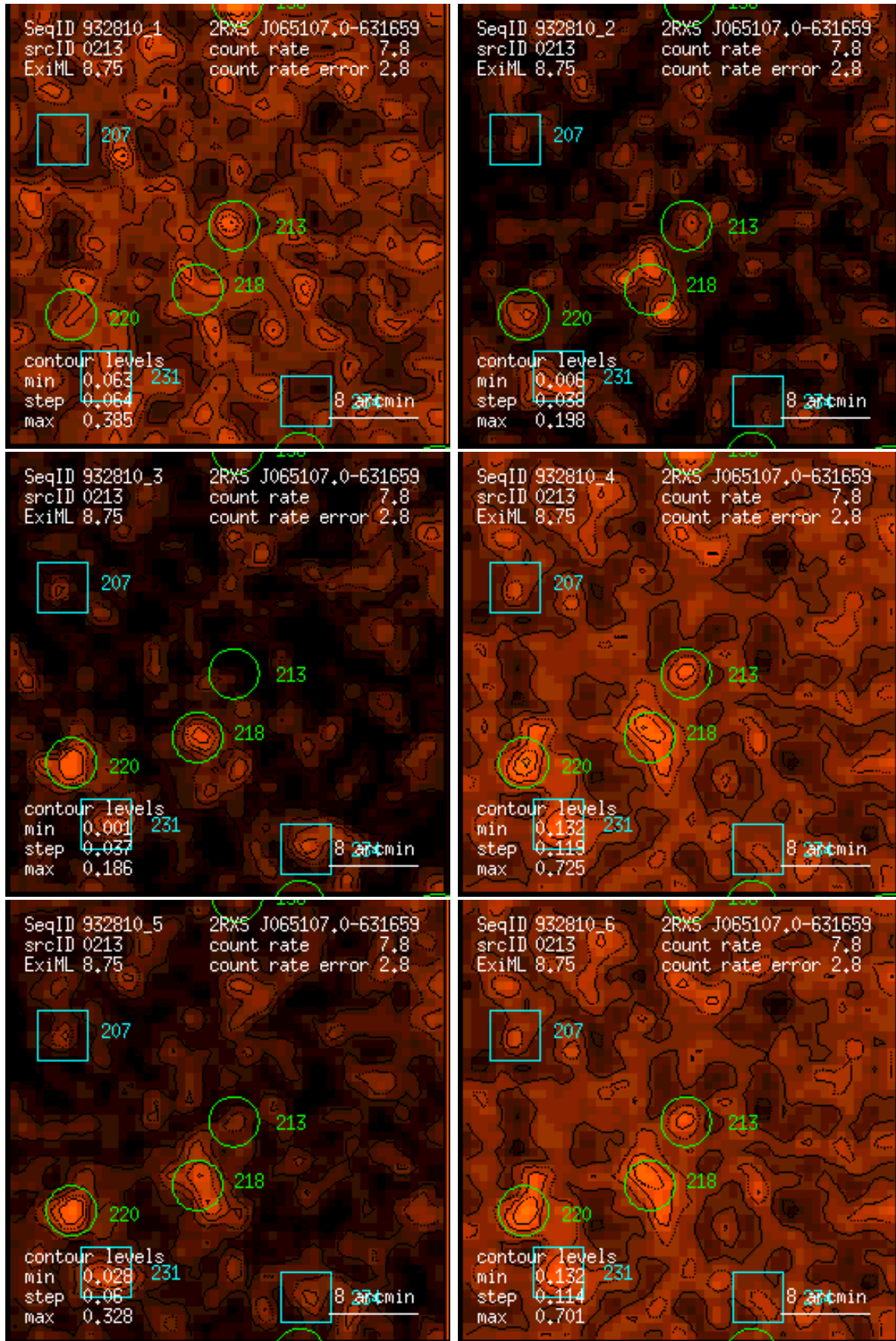
Figure 213: RASS 932810: detection 0213: band rate images, Gaussian filter: (1) PSPC channels 11 – 41, (2) 52 – 90, (3) 91 – 201, (4) 11 – 235, (5) 52 – 201, (6) 11 – 201. Broad band rates in counts/ks. Band rate contour levels in counts/ks/arcmin 2 .
