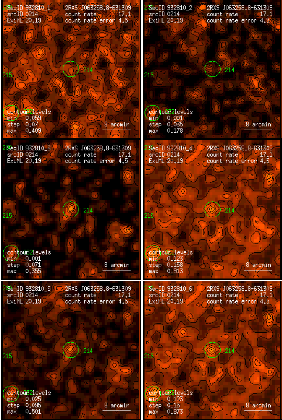
Figure 214: RASS 932810: detection 0214: band rate images, Gaussian filter: (1) PSPC channels 11 – 41, (2) 52 – 90, (3) 91 – 201, (4) 11 – 235, (5) 52 – 201, (6) 11 – 201. Broad band rates in counts/ks. Band rate contour levels in counts/ks/arcmin 2 .
