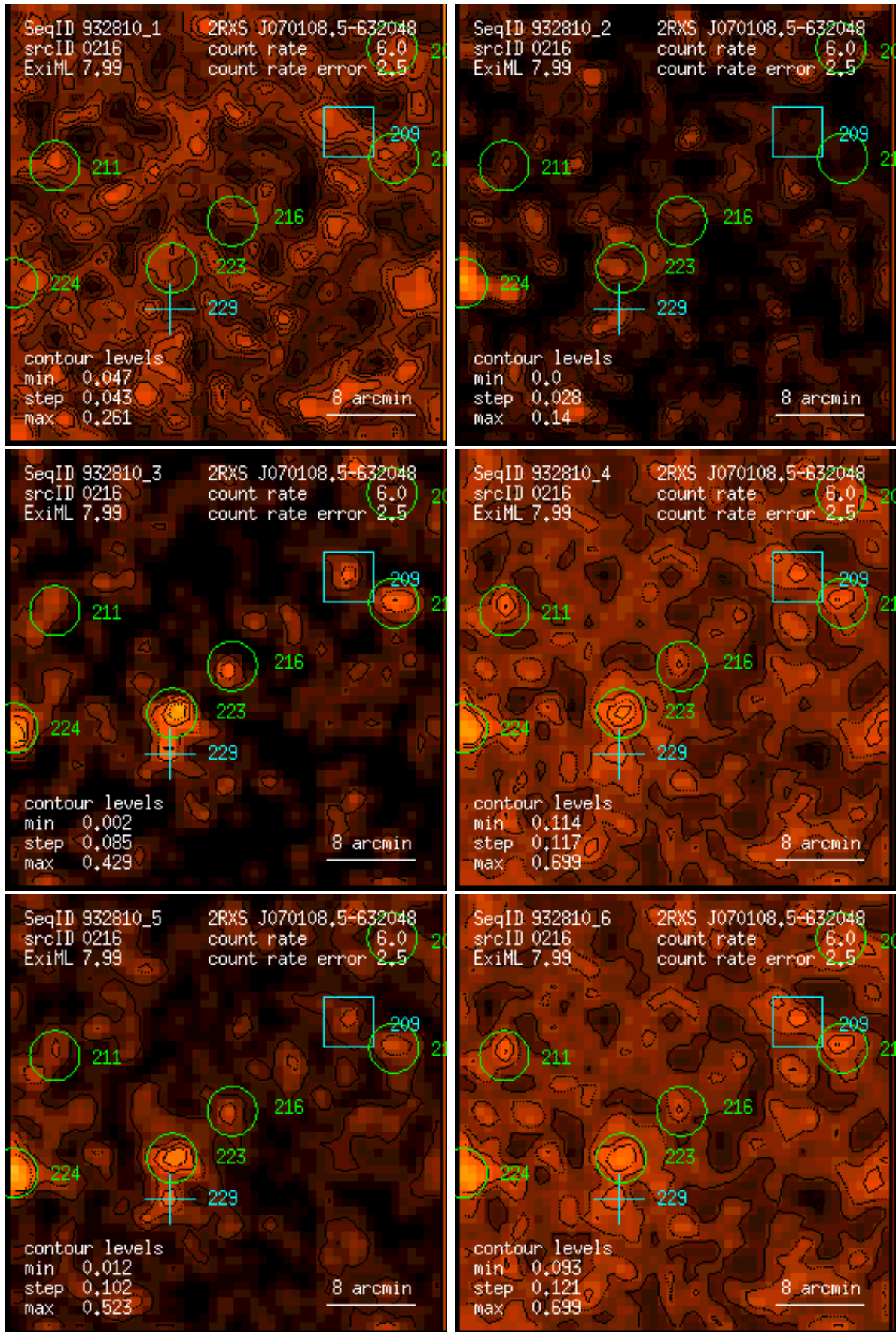
Figure 216: RASS 932810: detection 0216: band rate images, Gaussian filter: (1) PSPC channels 11 – 41, (2) 52 – 90, (3) 91 – 201, (4) 11 – 235, (5) 52 – 201, (6) 11 – 201. Broad band rates in counts/ks. Band rate contour levels in counts/ks/arcmin 2 .
