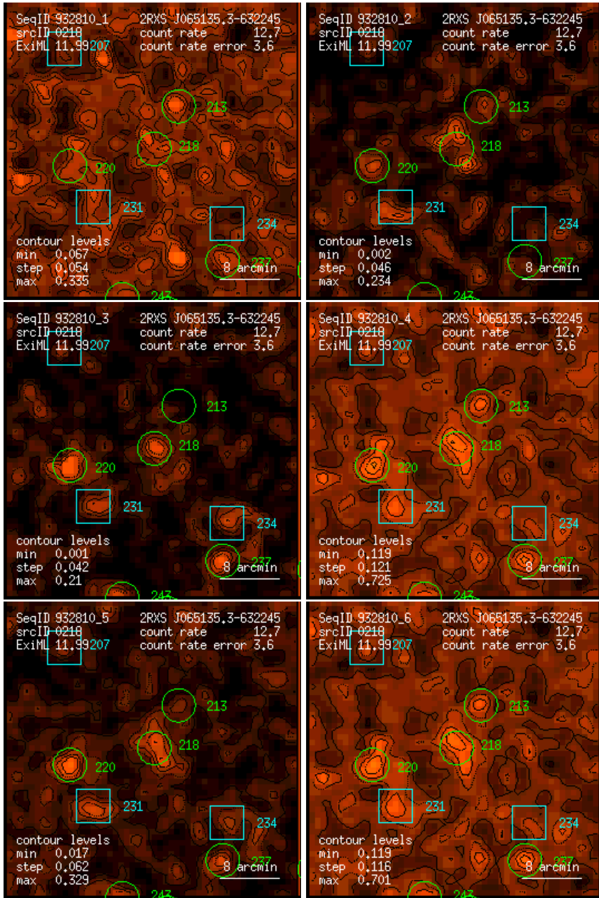
Figure 218: RASS 932810: detection 0218: band rate images, Gaussian filter: (1) PSPC channels 11 – 41, (2) 52 – 90, (3) 91 – 201, (4) 11 – 235, (5) 52 – 201, (6) 11 – 201. Broad band rates in counts/ks. Band rate contour levels in counts/ks/arcmin 2 .
