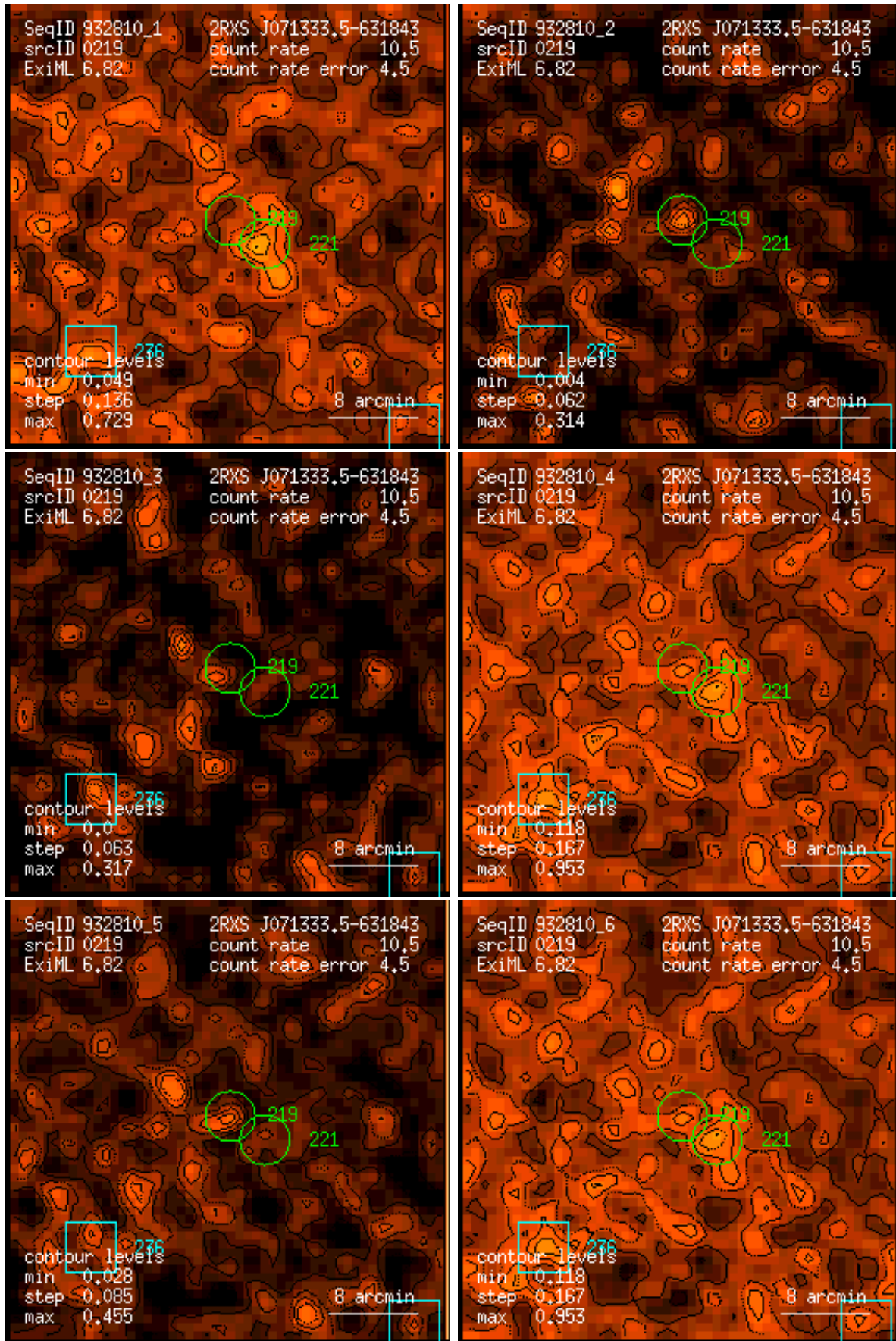
Figure 219: RASS 932810: detection 0219: band rate images, Gaussian filter: (1) PSPC channels 11 – 41, (2) 52 – 90, (3) 91 – 201, (4) 11 – 235, (5) 52 – 201, (6) 11 – 201. Broad band rates in counts/ks. Band rate contour levels in counts/ks/arcmin 2 .
