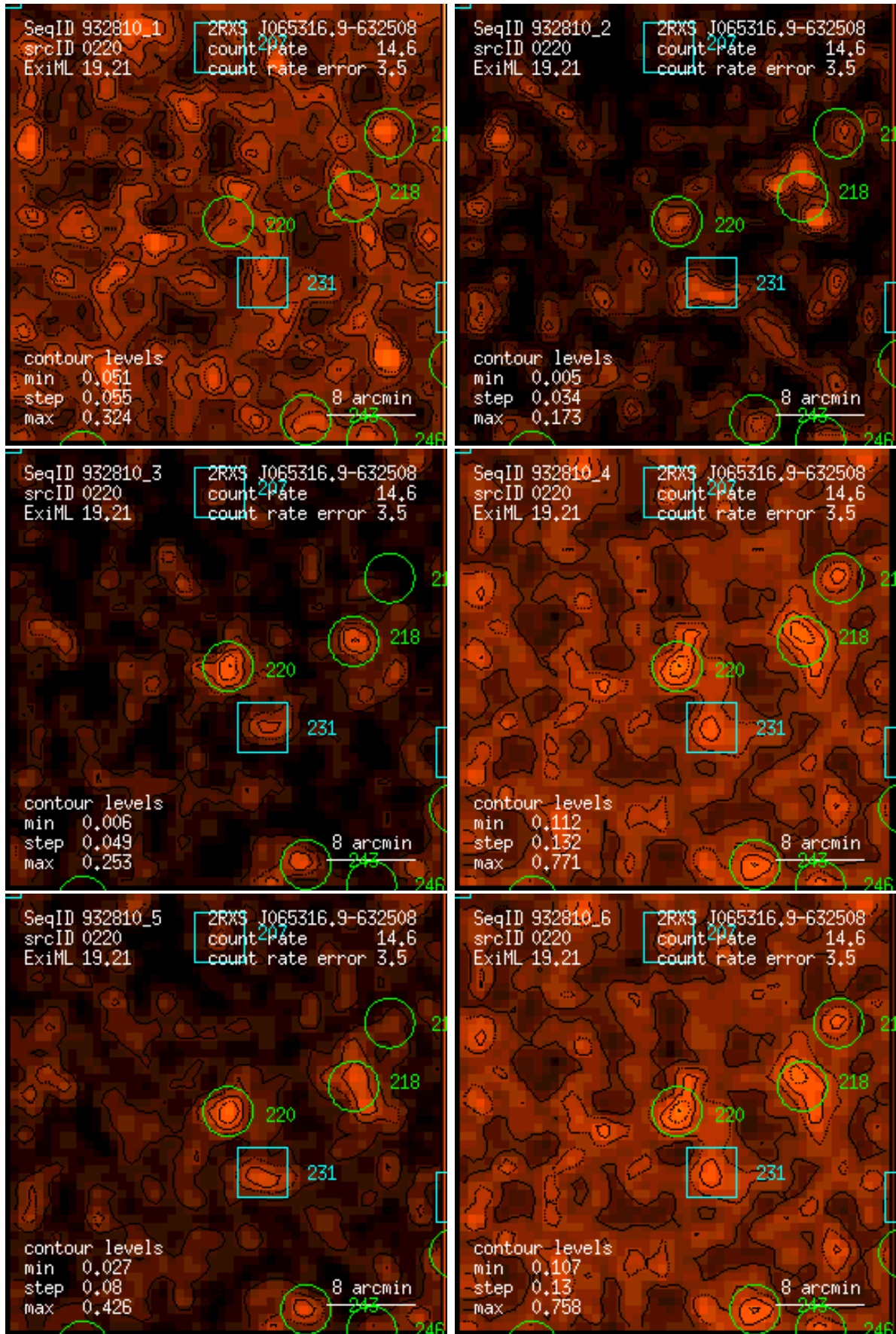
Figure 220: RASS 932810: detection 0220: band rate images, Gaussian filter: (1) PSPC channels 11 – 41, (2) 52 – 90, (3) 91 – 201, (4) 11 – 235, (5) 52 – 201, (6) 11 – 201. Broad band rates in counts/ks. Band rate contour levels in counts/ks/arcmin 2 .
