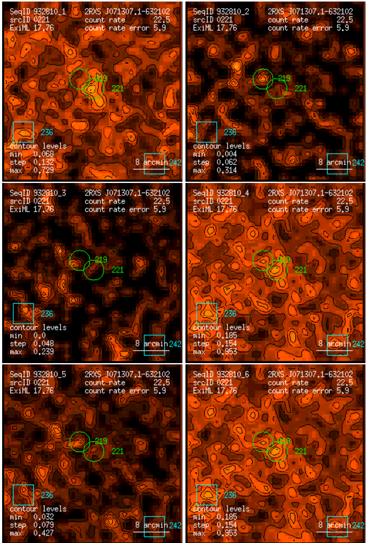
Figure 221: RASS 932810: detection 0221: band rate images, Gaussian filter: (1) PSPC channels 11 – 41, (2) 52 – 90, (3) 91 – 201, (4) 11 – 235, (5) 52 – 201, (6) 11 – 201. Broad band rates in counts/ks. Band rate contour levels in counts/ks/arcmin 2 .
