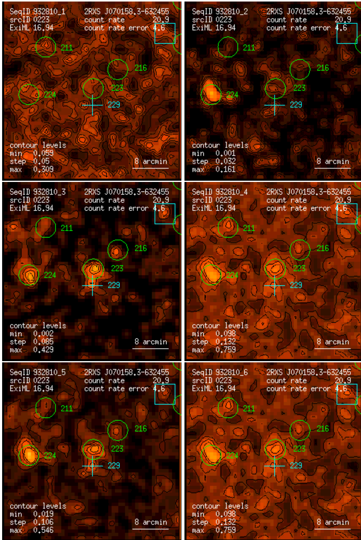
Figure 223: RASS 932810: detection 0223: band rate images, Gaussian filter: (1) PSPC channels 11 – 41, (2) 52 – 90, (3) 91 – 201, (4) 11 – 235, (5) 52 – 201, (6) 11 – 201. Broad band rates in counts/ks. Band rate contour levels in counts/ks/arcmin 2 .
