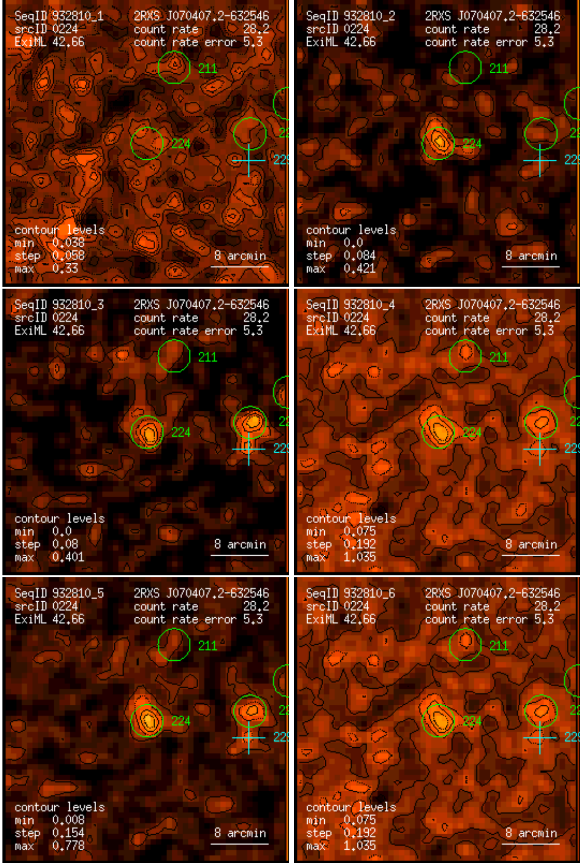
Figure 224: RASS 932810: detection 0224: band rate images, Gaussian filter: (1) PSPC channels 11 – 41, (2) 52 – 90, (3) 91 – 201, (4) 11 – 235, (5) 52 – 201, (6) 11 – 201. Broad band rates in counts/ks. Band rate contour levels in counts/ks/arcmin 2 .
