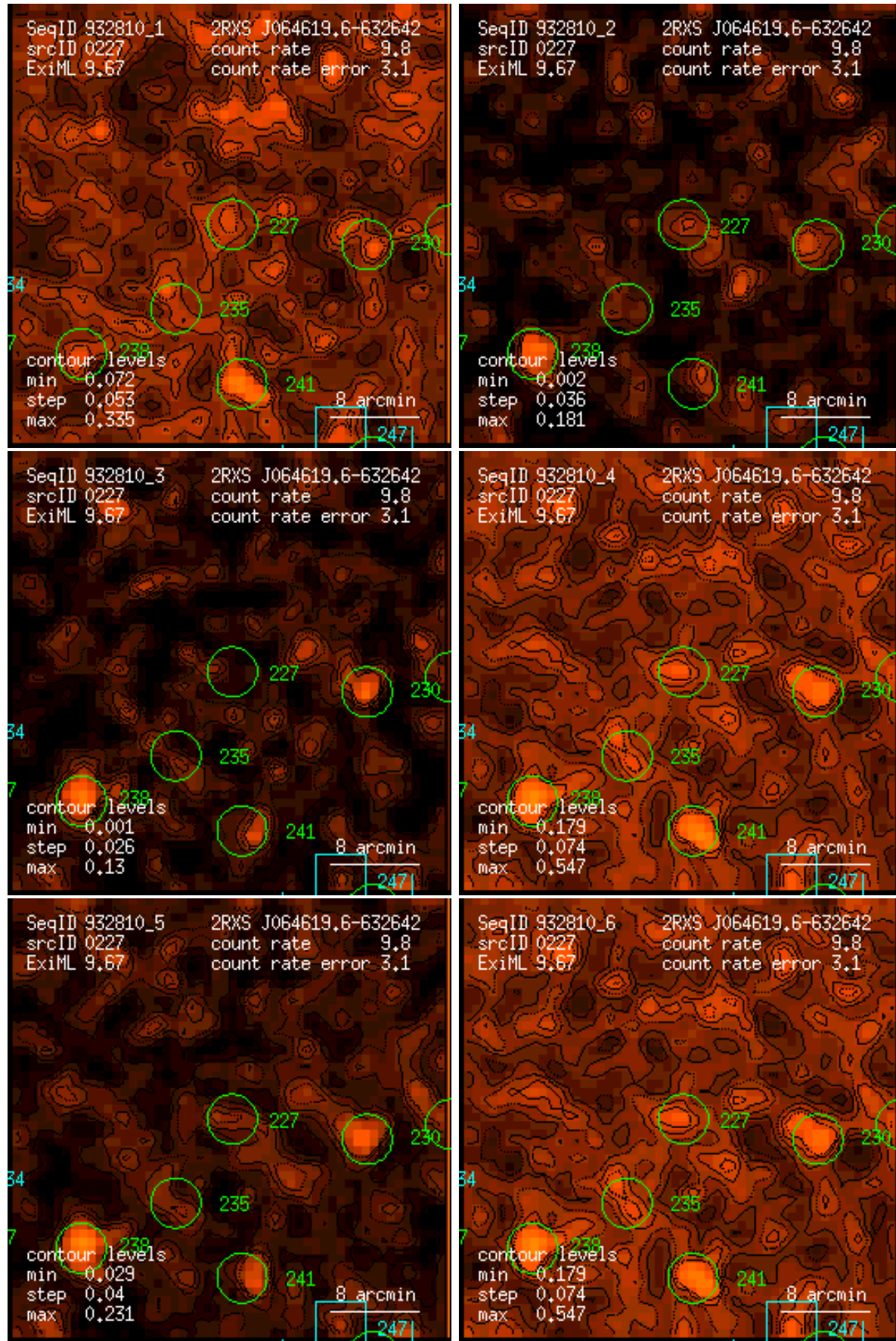
Figure 227: RASS 932810: detection 0227: band rate images, Gaussian filter: (1) PSPC channels 11 – 41, (2) 52 – 90, (3) 91 – 201, (4) 11 – 235, (5) 52 – 201, (6) 11 – 201. Broad band rates in counts/ks. Band rate contour levels in counts/ks/arcmin 2 .
