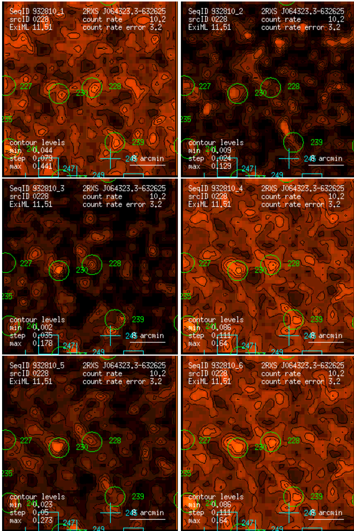
Figure 228: RASS 932810: detection 0228: band rate images, Gaussian filter: (1) PSPC channels 11 – 41, (2) 52 – 90, (3) 91 – 201, (4) 11 – 235, (5) 52 – 201, (6) 11 – 201. Broad band rates in counts/ks. Band rate contour levels in counts/ks/arcmin 2 .
