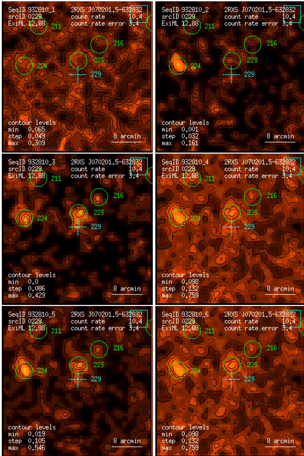
Figure 229: RASS 932810: detection 0229: band rate images, Gaussian filter: (1) PSPC channels 11 – 41, (2) 52 – 90, (3) 91 – 201, (4) 11 – 235, (5) 52 – 201, (6) 11 – 201. Broad band rates in counts/ks. Band rate contour levels in counts/ks/arcmin 2 .
