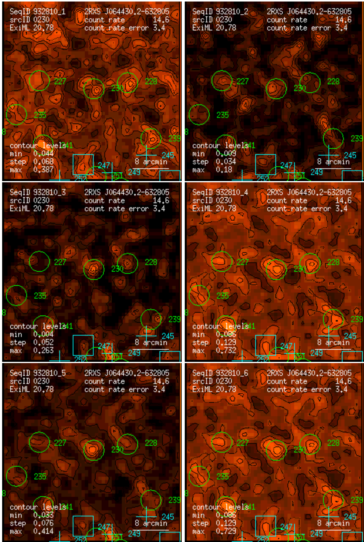
Figure 230: RASS 932810: detection 0230: band rate images, Gaussian filter: (1) PSPC channels 11 – 41, (2) 52 – 90, (3) 91 – 201, (4) 11 – 235, (5) 52 – 201, (6) 11 – 201. Broad band rates in counts/ks. Band rate contour levels in counts/ks/arcmin 2 .
