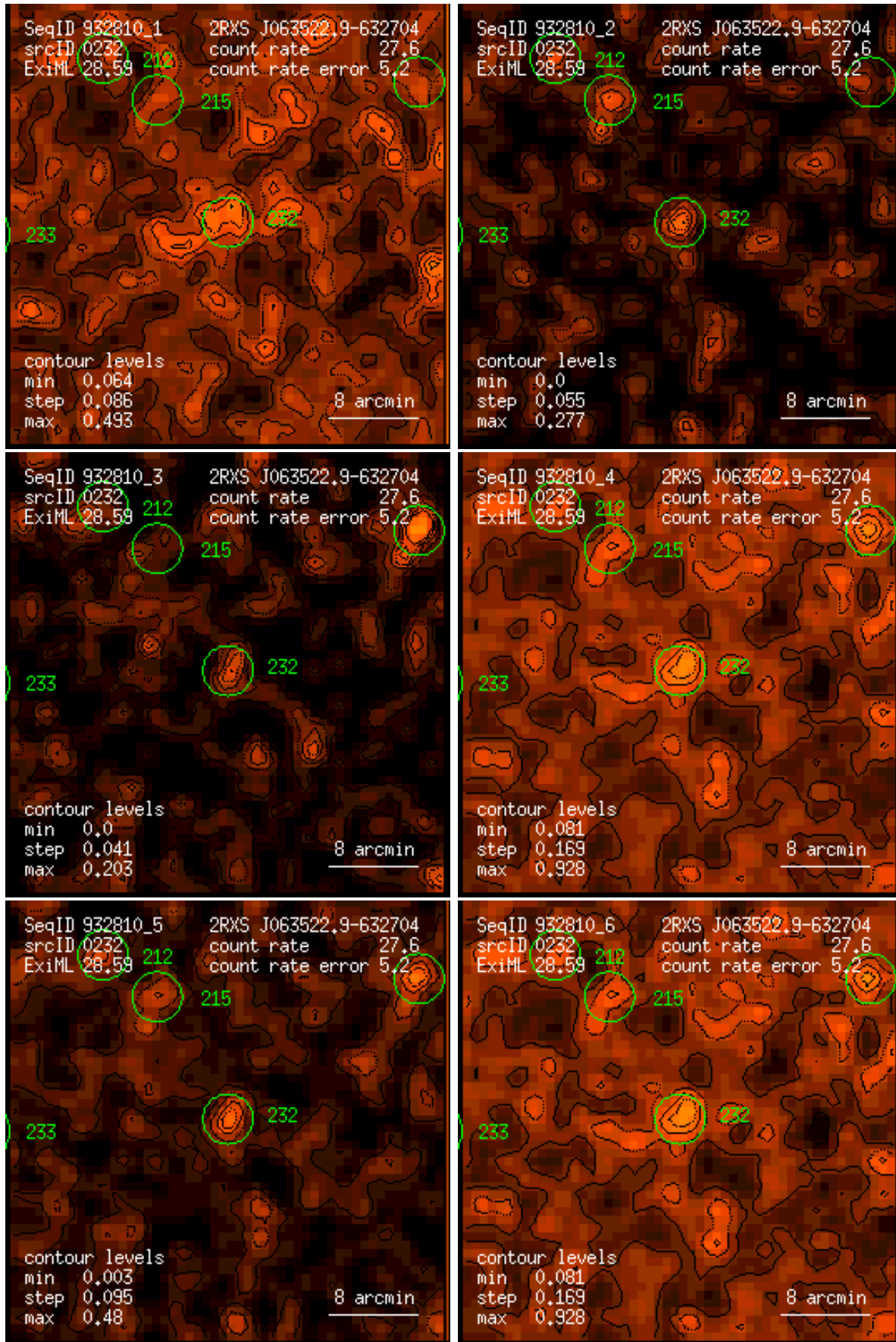
Figure 232: RASS 932810: detection 0232: band rate images, Gaussian filter: (1) PSPC channels 11 – 41, (2) 52 – 90, (3) 91 – 201, (4) 11 – 235, (5) 52 – 201, (6) 11 – 201. Broad band rates in counts/ks. Band rate contour levels in counts/ks/arcmin 2 .
