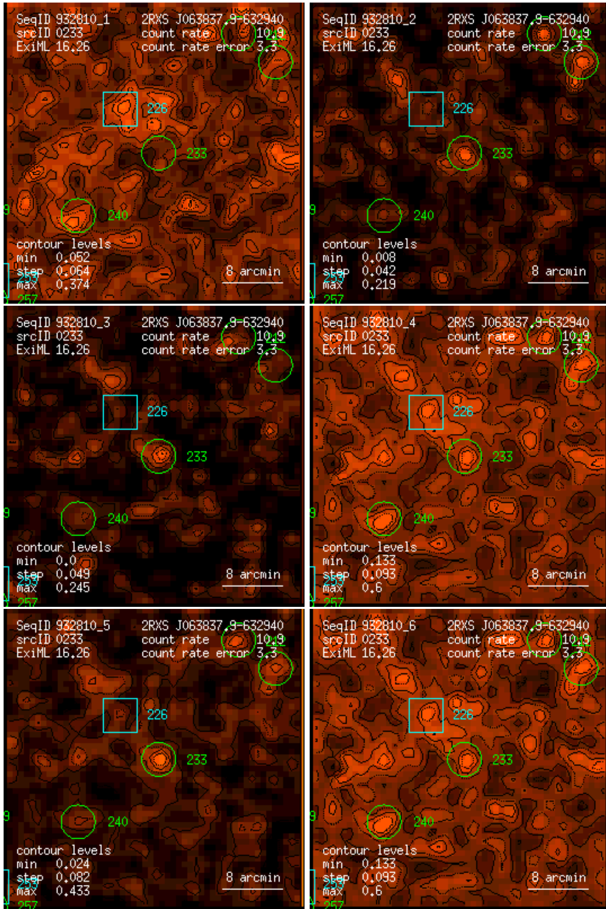
Figure 233: RASS 932810: detection 0233: band rate images, Gaussian filter: (1) PSPC channels 11 – 41, (2) 52 – 90, (3) 91 – 201, (4) 11 – 235, (5) 52 – 201, (6) 11 – 201. Broad band rates in counts/ks. Band rate contour levels in counts/ks/arcmin 2 .
